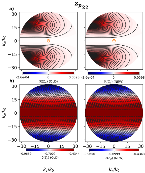
Fig. 6. Slow wave component of the plasma impedance matrix at 30 MHz: (a) Real part computed with the old and new versions of FELICE. (b) Imaginary part computed with the old and new versions of FELICE.
