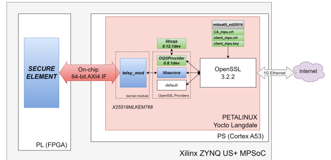
Fig. 3. Architecture of the MPU-based IoT device implementation.
