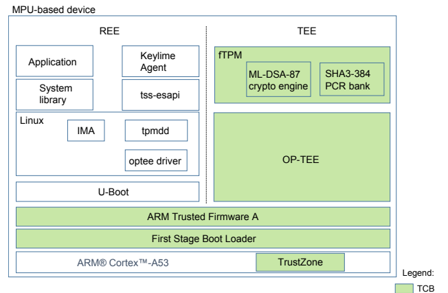
Fig. 5. Architecture of MPU-based IoT device for integrity verification. In the schema, the TCB of the designed architecture is highlighted in green.
