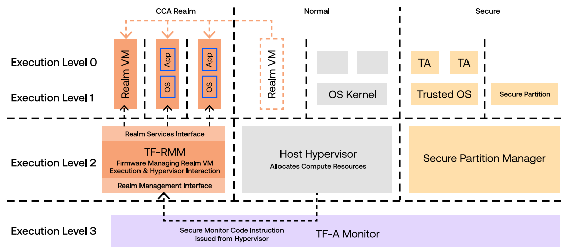
Figure 2: Arm Confidential Compute Architecture [26].
