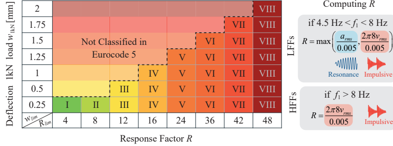
Fig. 1: Floor Performance levels according to the new version of Eurocode 5.
