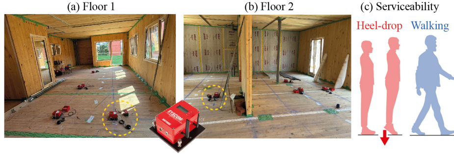
Fig. 3: (a) Floor 1. (b) Floor 2. (c) Vibration serviceability tests performed
