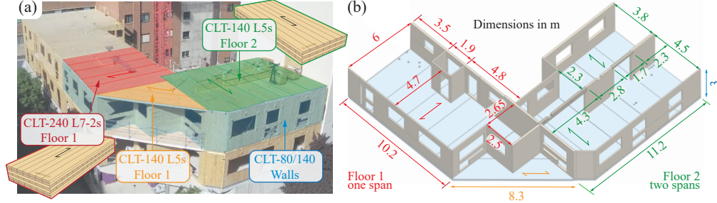
Fig. 2: (a) Different CLT panels used in the building structure. (b) Geometry of the floor.
