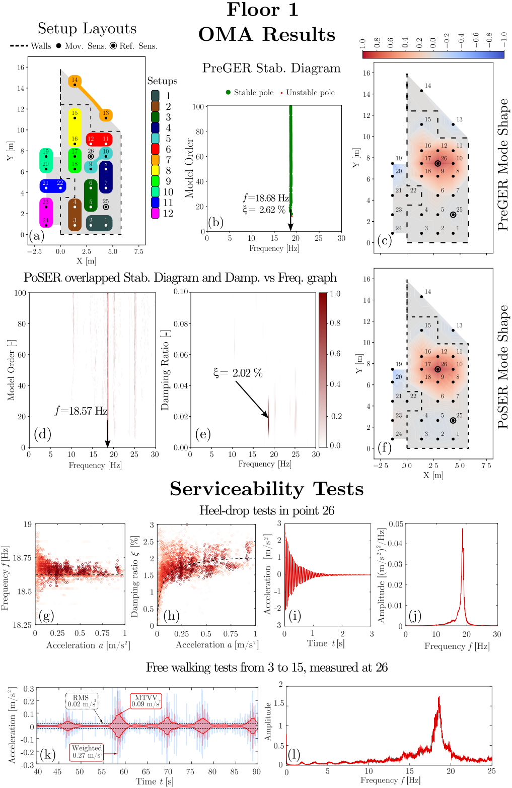
Fig. 4: OMA and serviceability results for floor 1.
