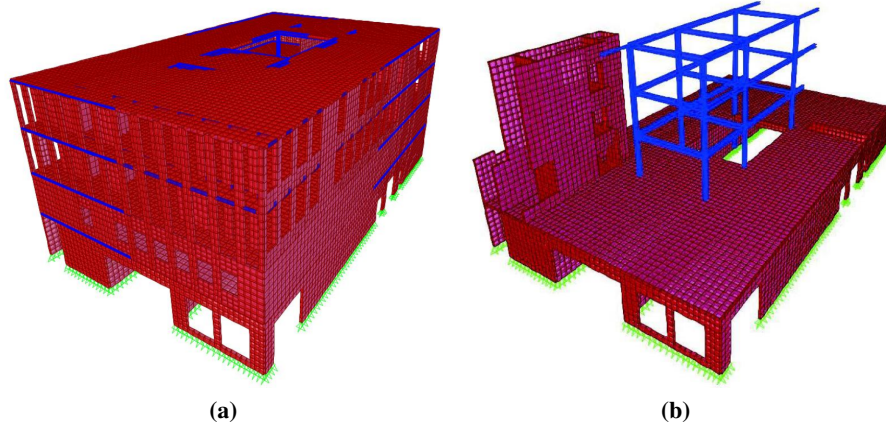
Fig. 4. Numerical global FEM implemented model. (a) a visualization of the FEM model in CSI SAP2000 software; (b) the FEM detailing of an internal steel framing system into the central part of the building.
