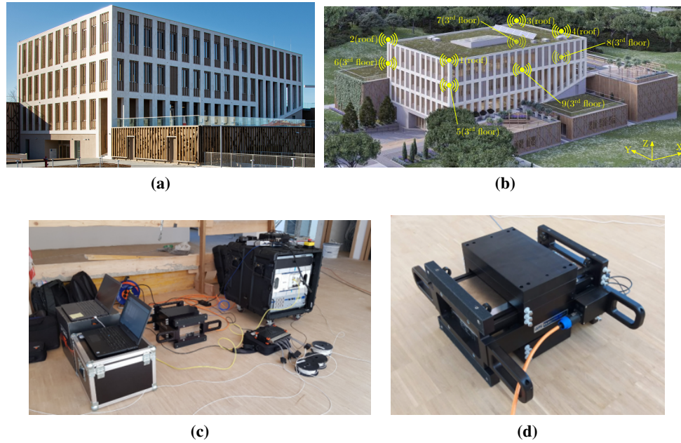
Fig. 1. Case study overview. (a) a photo of the monitored building; (b) the deployed accelerometer layout; (c) a photo of the vibration monitoring system; (d) a photo of the shaker used for forced vibration tests.
