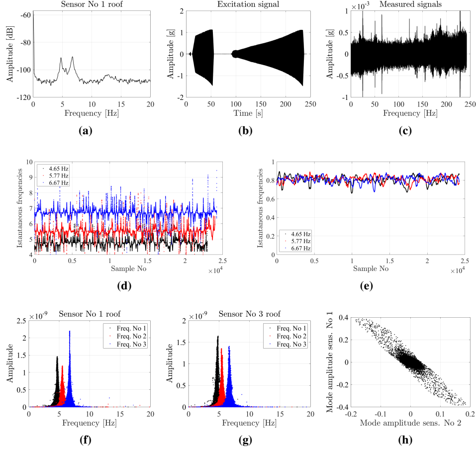
Fig. 3. Forced vibration test results. (a) PSD of a reference sensor; (b) shaker input excitation signal; (c) sensors measured signals during forced tests; (d) IF for the first three modes; (e) Modal Assurance Criterion metric among the IF of the first three modes; (f) IA vs IF graphs for sensor No 1 on the roof; (g) IA vs IF graphs for sensor No 3 on the roof; (h) correlation between IA of sensors No 1 vs No 2 .
