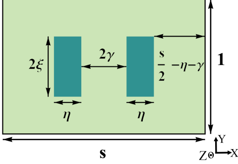
Fig. 1. The unit cell. The selected geometrical structure features two symmetrically positioned windows with a permittivity distinct from that of the surrounding background. All geometrical parameters are dimensionless and normalized by l_y , the vertical edge length of the unit cell. The unit cell is not required to be square, as indicated when s \neq 1 . For this study, we choose to set s = 1 .
