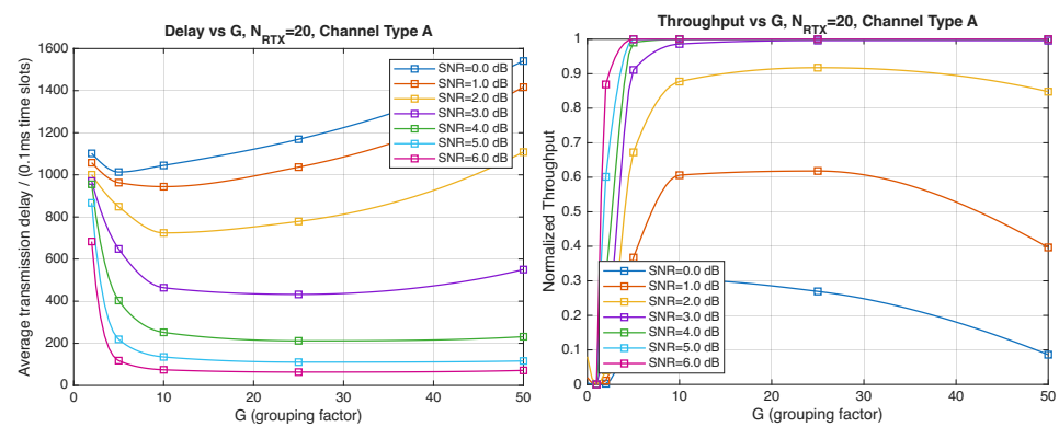
Figure 13. Average transmission delay of successful packets and normalized throughput with HARQ-I versus G for N_{\text{RTX}} = 20 (Channel type A, \mu = 13 , (Low rate), R_c = \frac{1}{2} , N_{\Delta} = 100 ).
