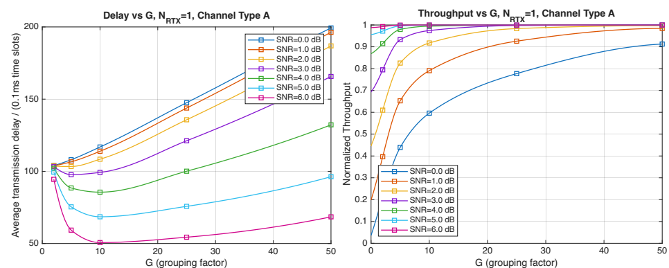
Figure 14. Average transmission delay of successful packets and normalized throughput with HARQ-II versus G for N_{\text{RTX}} = 1 (Channel type A, \mu = 13 , (Low rate), R_c = \frac{1}{2} , N_{\Delta} = 100 ).
