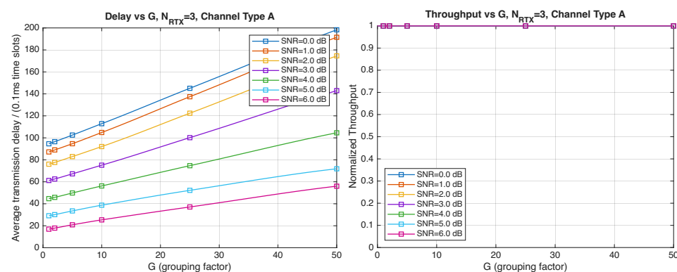
Figure 11. Average transmission delay of successful packets and normalized throughput with HARQ-II versus G for N_{\text{RTX}} = 3 (Channel type A, \mu = 0 , (High rate), R_c = \frac{1}{2} , N_\Delta = 100 ).
