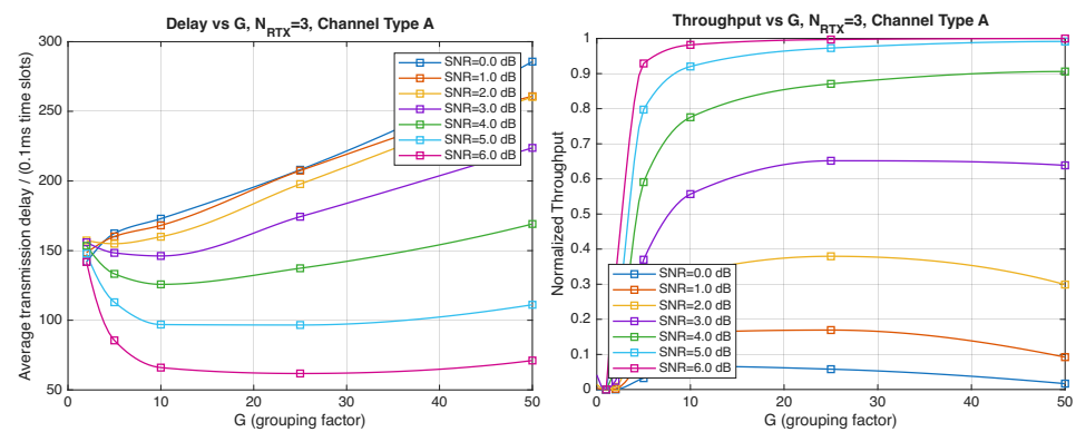
Figure 12. Average transmission delay of successful packets and normalized throughput with HARQ-I versus G for N_{\text{RTX}} = 3 (Channel type A, \mu = 13 , (Low rate), R_c = \frac{1}{2} , N_{\Delta} = 100 ).
