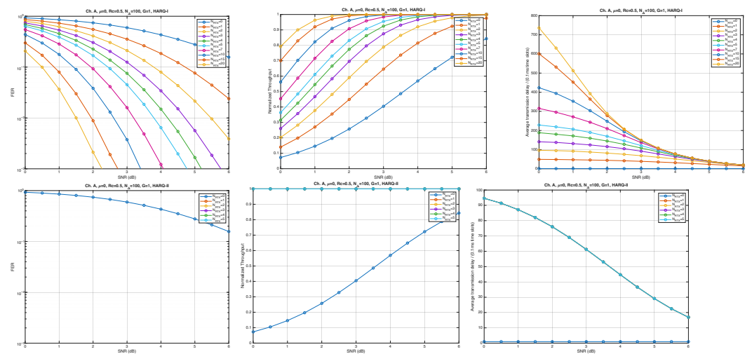
Figure 5. Plots of FER, Throughput, and Delay versus SNR. Channel A, \mu = 0 , R_c = \frac{1}{2} , N_{\Delta} = 100 , G = 1 , and different values of the maximum number of retransmissions allowed N_{\text{RTX}} . Upper row: HARQ-I. Lower row: HARQ-II. Some curves in the lower row (HARQ-II) overlap, meaning that from a certain value of N_{\text{RTX}} on, the performance does not change.
