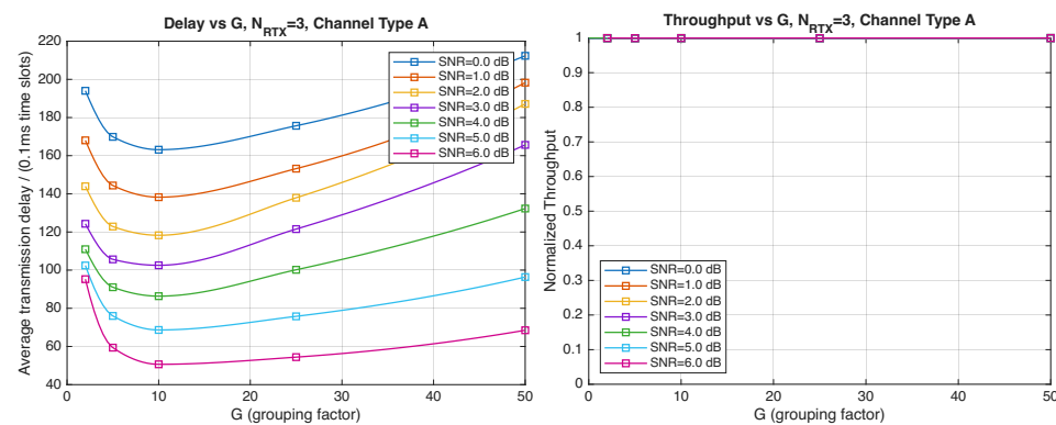
Figure 15. Average transmission delay of successful packets and normalized throughput with HARQ-II versus G for N_{\text{RTX}} = 3 (Channel type A, \mu = 13 , (Low rate), R_c = \frac{1}{2} , N_\Delta = 100 ).
