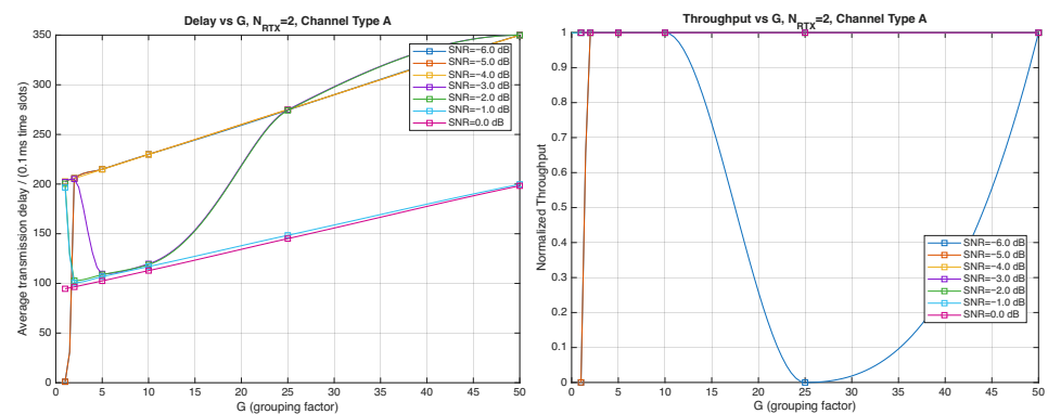
Figure 21. Average transmission delay of successful packets and normalized throughput with HARQ-II versus G for N_{\text{RTX}} = 2 (Channel type A, \mu = 0 , R_c = \frac{1}{2} , N_\Delta = 100 , very low SNR).
