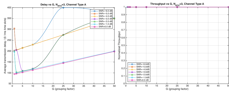
Figure 22. Average transmission delay of successful packets and normalized throughput with HARQ-II versus G for N_{\text{RTX}} = 3 (Channel type A, \mu = 0 , R_c = \frac{1}{2} , N_\Delta = 100 , very low SNR).
