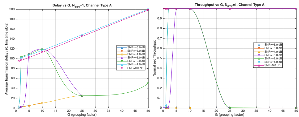
Figure 20. Average transmission delay of successful packets and normalized throughput with HARQ-II versus G for N_{\text{RTX}} = 1 (Channel type A, \mu = 0 , R_c = \frac{1}{2} , N_\Delta = 100 , very low SNR).
