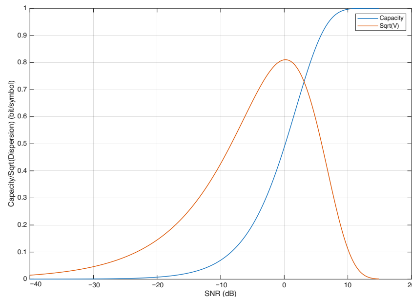
Figure 3. Mutual information and square root of the channel dispersion vs. SNR.
