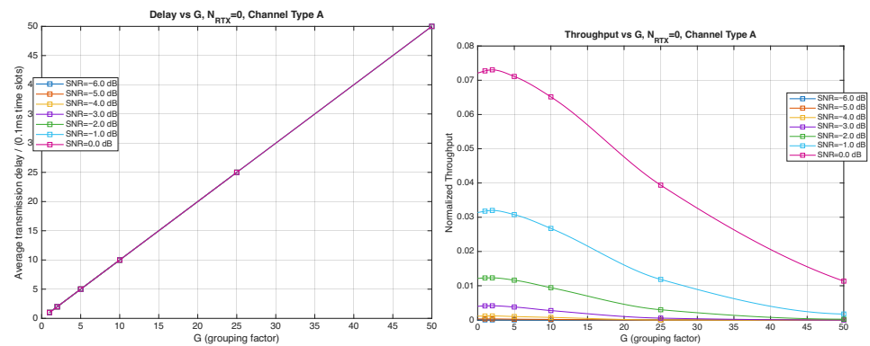
Figure 19. Average transmission delay of successful packets and normalized throughput with HARQ-II versus G for N_{\text{RTX}} = 0 (Channel type A, \mu = 0 , R_c = \frac{1}{2} , N_\Delta = 100 , very low SNR).
