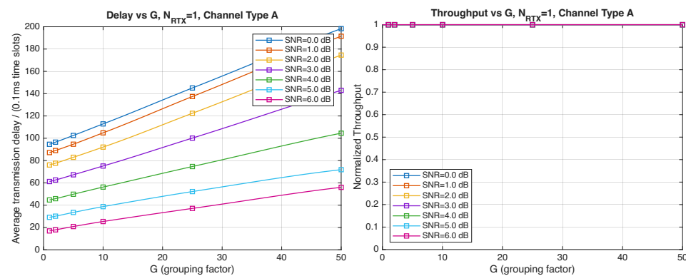
Figure 10. Average transmission delay of successful packets and normalized throughput with HARQ-II versus G for N_{\text{RTX}} = 1 (Channel type A, \mu = 0 , (High rate), R_c = \frac{1}{2} , N_\Delta = 100 ).
