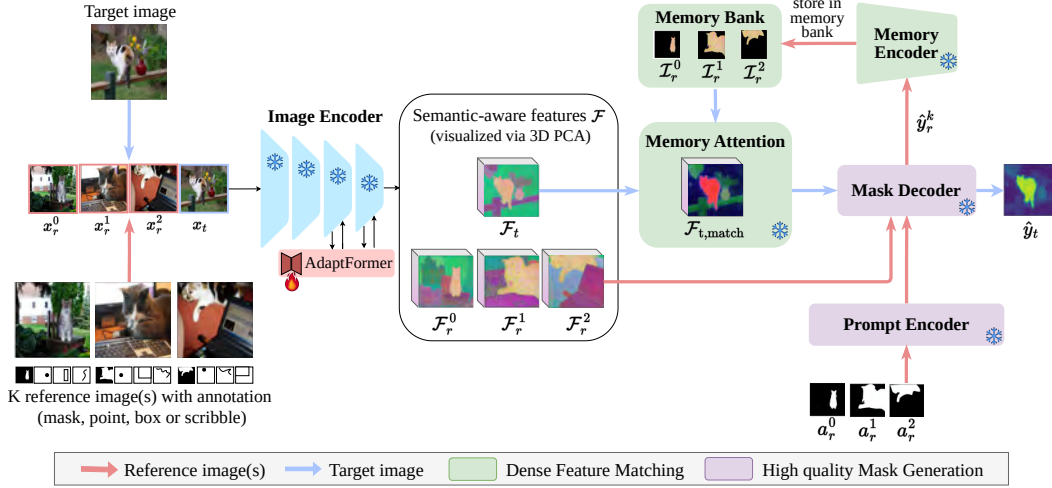
Figure 3: Overview of SANSa: Given k annotated reference images and a target image, we construct a pseudo-video by concatenating them, then leverage SAM2 streaming pipeline to process reference frames together with their annotations sequentially. We restructure SAM2 feature space to make its latent semantic structure explicit , enabling mask propagation based on semantic similarity from reference to target. The emergent semantic structure is visualized by the 3D PCA projection of \mathcal{F} .
