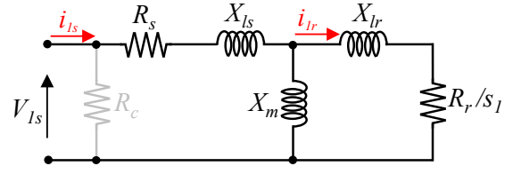
(a) Equivalent circuit for the fundamental harmonic.
