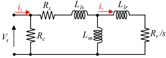
Fig. 1: Single-phase simplified equivalent circuit.
