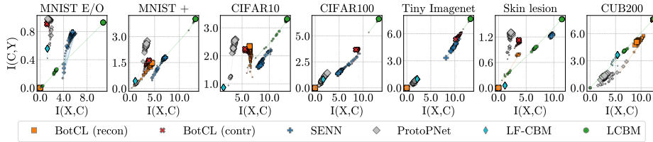
Fig. 5: Information Plane for the different models in terms of Mutual information between concept and input variables I(X,C) , and between the concept and output variables I(C,Y) . The size of the markers is proportional to the training epoch.
