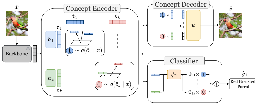
Fig. 3: LCBM schema. The concept encoder q(c | x) provides the probability for each learnt concept \hat{c}_j and the associated embeddings \mathbf{c}_j . Both concept scores and embeddings are used to predict the output class p(y | c) and to reconstruct the input p(x | c) .
