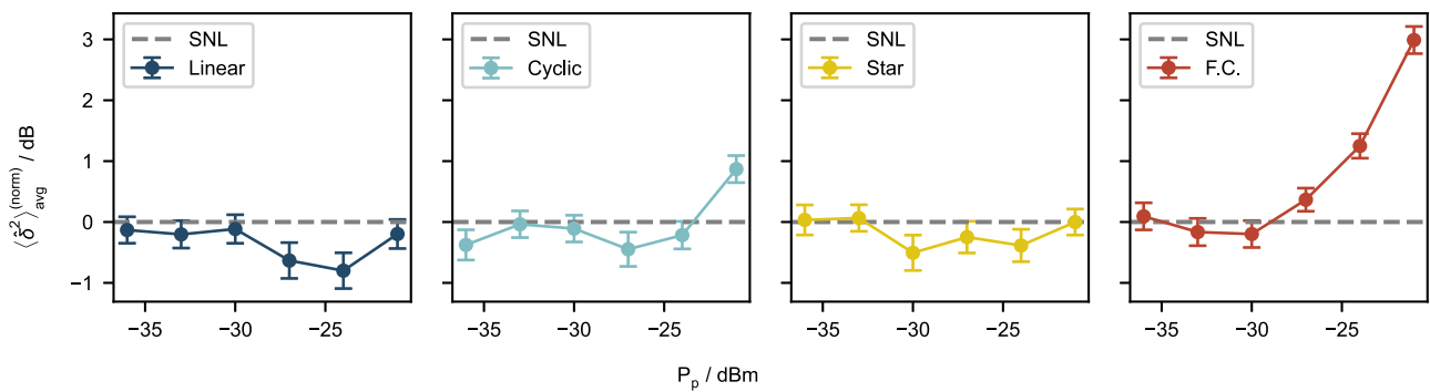
Fig. 2 | Cluster quality metrics for different topologies and pump powers. Dependence of the average nullifier variance, normalized to the shot noise level (SNL), \langle \delta^2 \rangle_{\text{avg}}^{(\text{norm})} , on the power P_p of a single pump tone (identical for all pairs),
