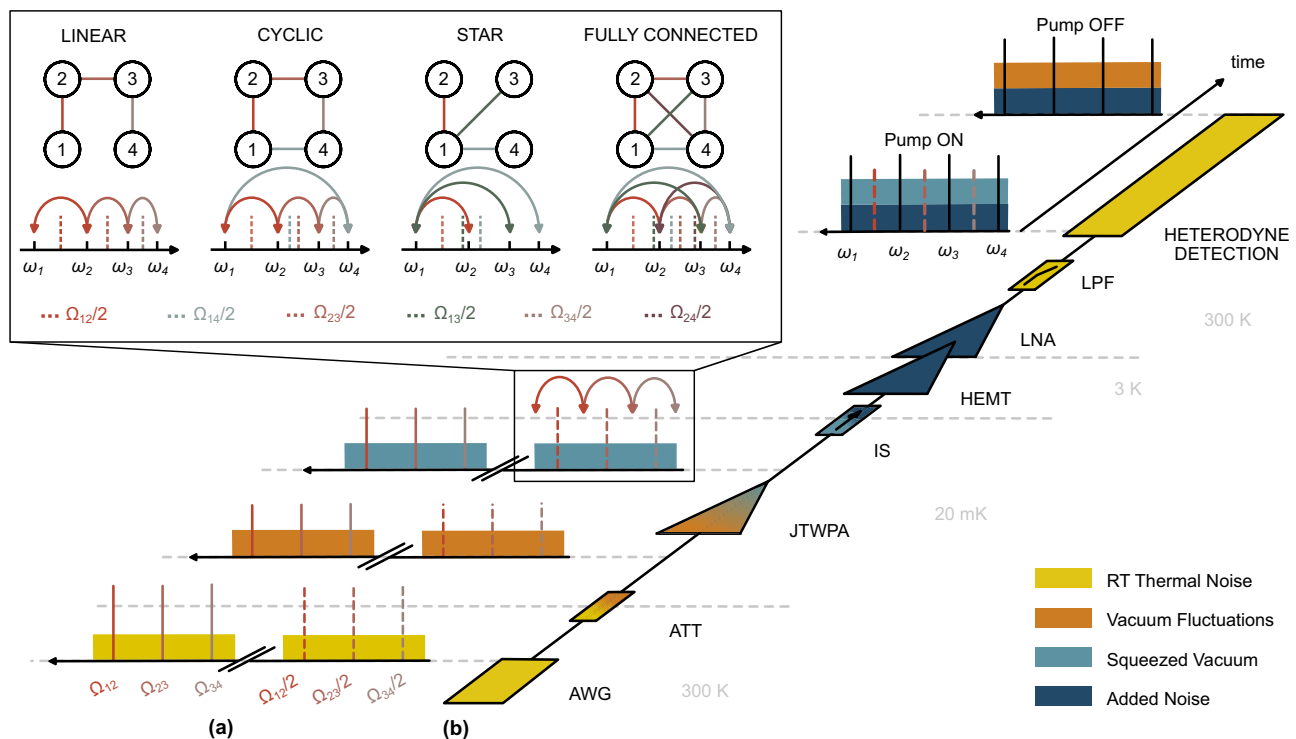
Fig. 1 | Programmable generation of microwave cluster states using a Josephson Traveling-Wave Parametric Amplifier (JTWP). a Frequency-domain continuous-variable (CV) cluster-state protocol. Multiple non-equidistant pump tones at frequencies \Omega_{jl} drive the JTWP in the three-wave mixing regime, implementing two-mode squeezing interactions between vacuum modes at frequencies \omega_j and \omega_l . The interaction transforms input vacuum fluctuations into two-mode squeezed vacuum states, while thermal noise from room-temperature (RT) components is suppressed by cryogenic attenuation. The detection scheme employs a pump ON/
