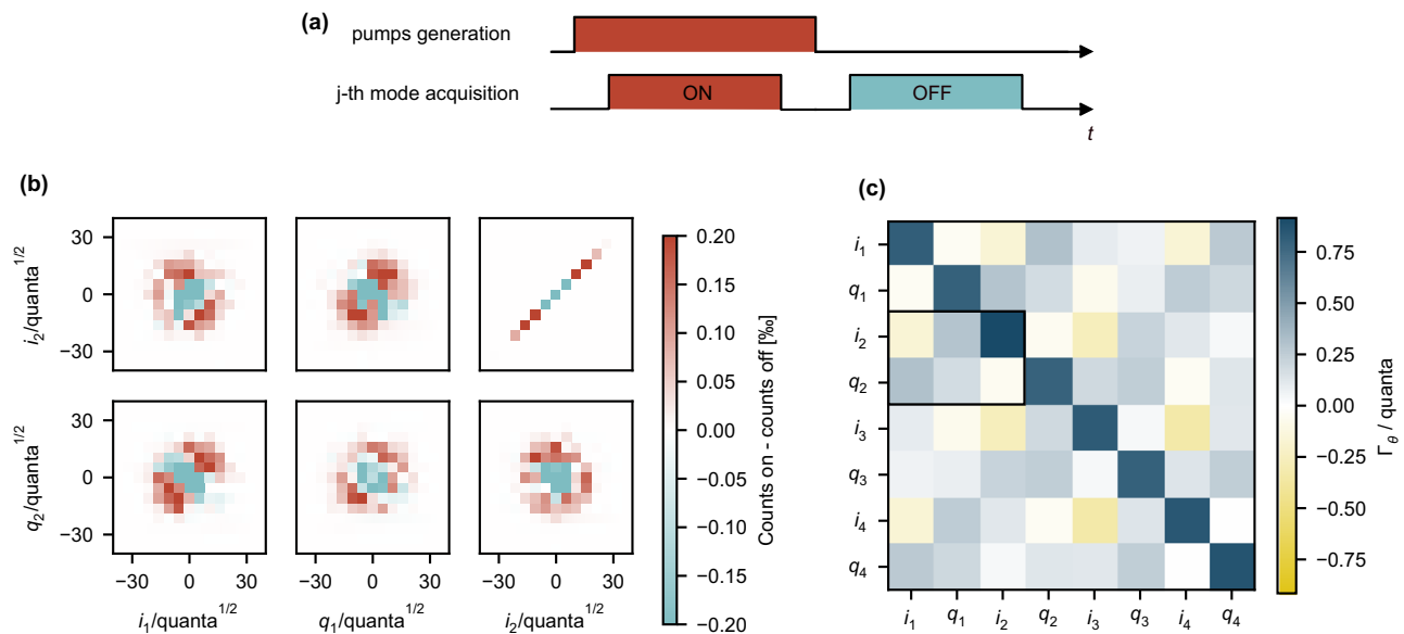
Fig. 4 | Gaussian cluster state covariance matrix reconstruction. a Scheme of the pumps interleaved generation via an ON-OFF protocol, which guarantees referenced-state multiplexed heterodyne detection of modes. b Histograms reporting the counts of quadratures measured in the ON condition, subtracted using the reference state acquired during the OFF state for modes 1 and 2.
