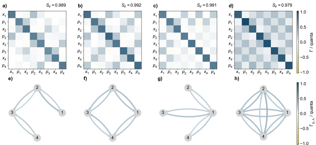
Fig. 3 | Quadrature covariance matrices and inferred graph connectivity. a–d Reconstructed covariance matrix \Gamma of the quadrature operators at P_p = -24 dBm, extracted from heterodyne detection of four frequency modes clustered in linear ( a , e ), cyclic ( b , f ), star ( c , g ), and fully-connected ( d , h )
