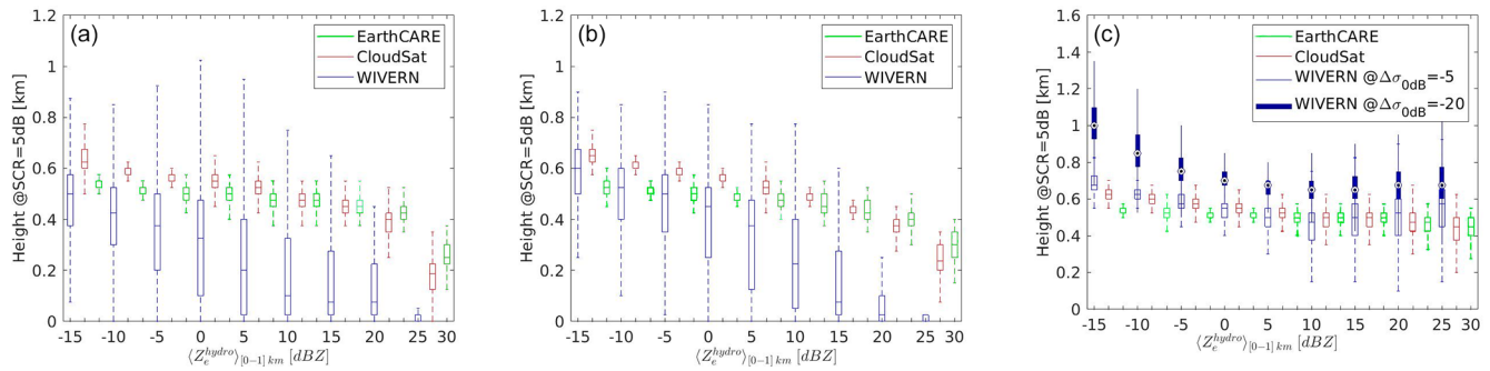
Figure 13. Boxplots of the distributions of H_{SCR=5\text{ dB}} as a function of the mean value of \langle Z_e^{\text{hydro}} \rangle_{[0-1]\text{ km}} for oceanic rainfall (a), snowfall (b), and snowfall over land or sea ice (c). In the boxplots, the central mark indicates the median, and the bottom and top edges of the box indicate the 25th and 75th percentiles, respectively, whereas the whiskers extend to the most extreme data points not considered to be outliers. In panel (c), there are two boxplots for the WIVERN corresponding to \Delta\sigma_0 = -5 and 20 dB, respectively.
