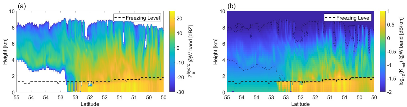
Figure 6. W-band vertical profiles of effective reflectivity (a) and W-band hydrometeor extinction coefficient (b) corresponding to the microphysical properties shown in Fig. 5. The dashed black line corresponds to the freezing level.
