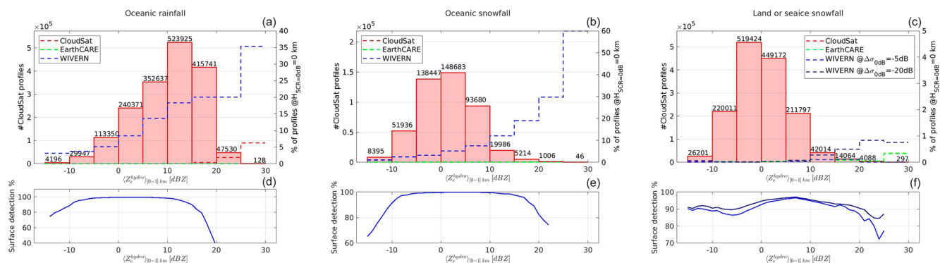
Figure 14. (a–c) Number of CloudSat profiles selected for statistical analysis: for oceanic rainfall on the left, oceanic snowfall in the middle panel, and land or sea ice snowfall on the right; profiles are clustered by effective reflectivity into surface classes from -15 to 30 dBZ, each 5 dBZ wide. Dashed lines are the percentage of profiles detected at ground level ( H_{\text{SCR}=5\text{dB}} = 0 \text{ km} ) and are shown for the WIVERN (blue), CloudSat (red), and EarthCARE (magenta). (d–f) Proportion of profiles detected by the WIVERN compared to those detected by CloudSat as a function of \langle Z_e^{\text{hydro}} \rangle_{[0-1]\text{km}} . The profiles detected by CloudSat are the 100\% baseline. Results are only shown for reflectivity classes with more than 100 profiles.
