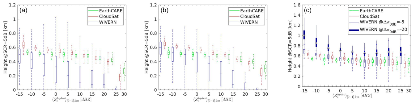
Figure 13. Boxplots of the distributions of H_{\text{SCR}=5\text{dB}} as a function of the mean value of \langle Z_e^{\text{hydro}} \rangle_{[0-1]\text{km}} for oceanic rainfall (a), snowfall (b), and snowfall over land or sea ice (c). In the boxplots, the central mark indicates the median, and the bottom and top edges of the box indicate the 25th and 75th percentiles, respectively, whereas the whiskers extend to the most extreme data points not considered to be outliers. In panel (c), there are two boxplots for the WIVERN corresponding to \Delta\sigma_0 = -5 and 20 dB, respectively.
