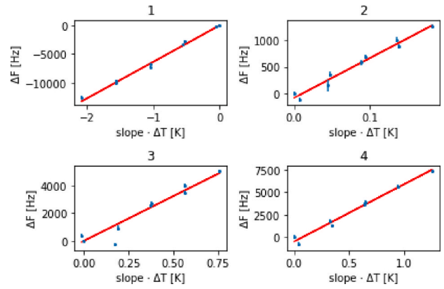
Fig. 7. 4 calibration curves obtained decreasing and increasing the temperature of the incubator enclosing the experimental setup in a Faraday cage.
