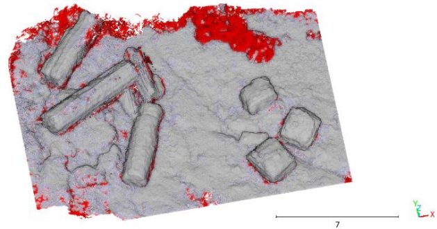
Figure 10. Data completeness result for the 3DGS-PostShot point cloud. Red points represent the missing parts.
