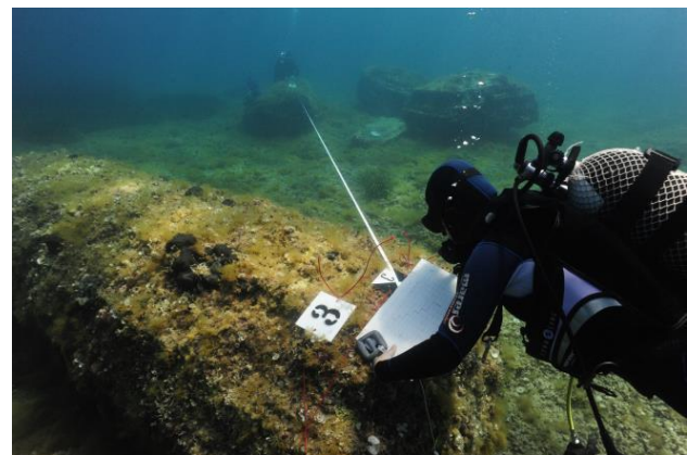
Figure 3. Trilateration operations for the GCPs measuring.
