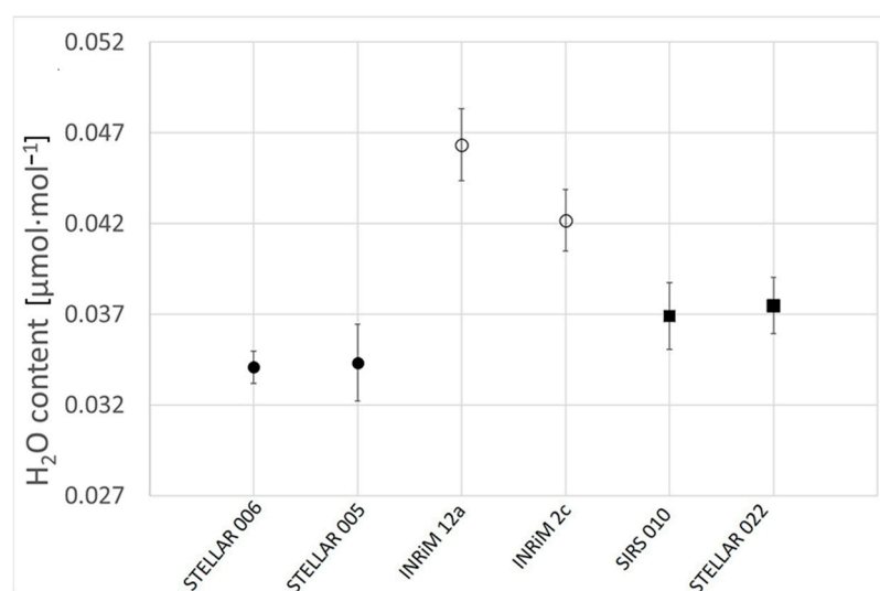
Figure 7. Comparison of the results obtained for the H 2 O content ( \mu\text{mol}\cdot\text{mol}^{-1} ) in different CO 2 in air reference gas mixtures, measured using CRDS. Different symbols are used to denote pairs of mixtures having similar matrices and preparation dates.
