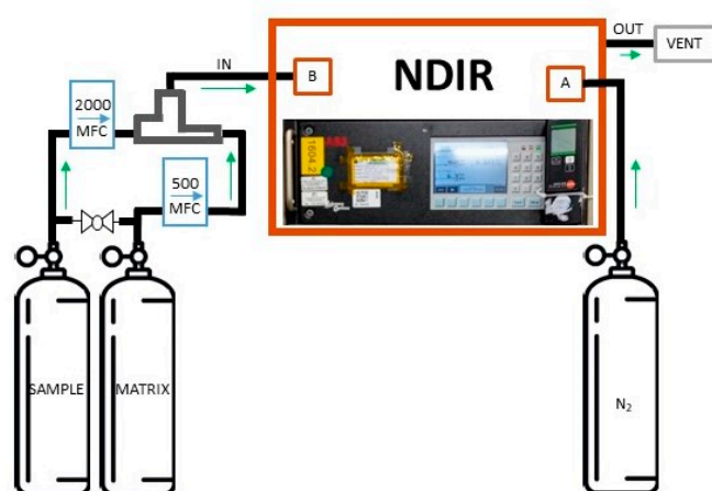
Figure 2. Schematic representation of the set-up of the NDIR analyzer URAS 14 (ABB, Switzerland) for the analysis of CO 2 amount fractions in pure Ar.
