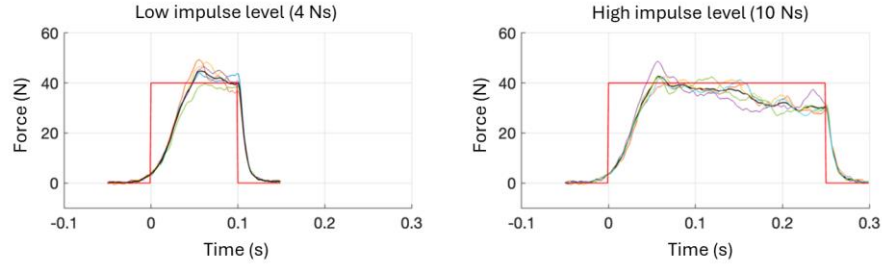
Fig. 3. Perturbation profiles exerted on a subject for low and high impulse values: red thick line is the reference force signal; black thick line is the average signal measured by the load cell over a set of consecutive perturbations shown in thin colored lines.
