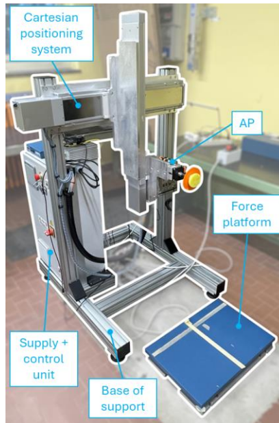
Fig. 1. The complete automated perturbation system (aPGAS).
