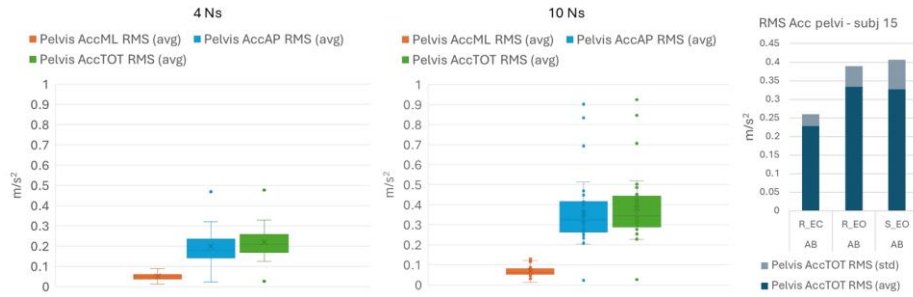
Fig. 5. RMS values of pelvis accelerations for low (left) and high (center) impulse levels averaged across all subjects, RMS values for a specific subject in the three conditions tested (right). ML = medio-lateral, AP = anteroposterior, TOT = total.
