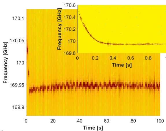
Figure 3. Spectrogram showing the instantaneous gyrotron frequency during 100 s long gyrotron pulse. The variation of the measured spectral maximum in frequency is of max. \pm 6 MHz after a stabilisation time of 20 seconds.
