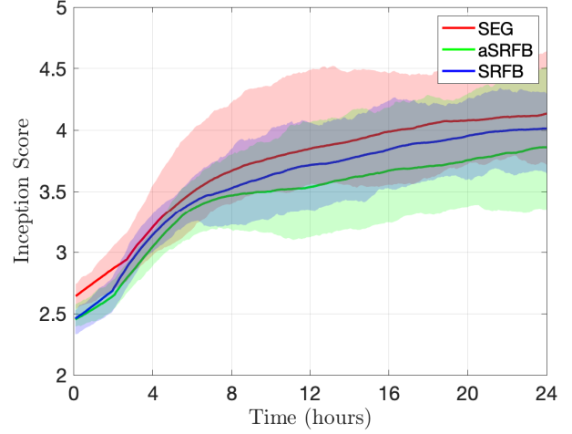
Fig. 1: Inception scores reached by the EG, the SRFB and the aSRFB algorithms.
