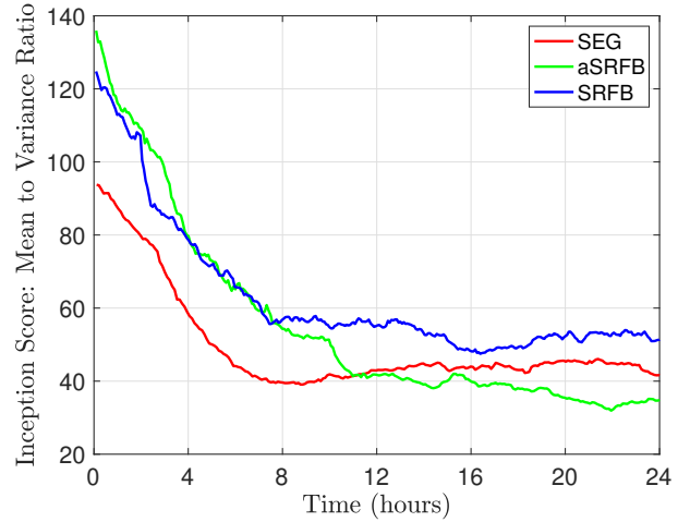
Fig. 2: Mean to variance ratio corresponding to the average inception scores.
