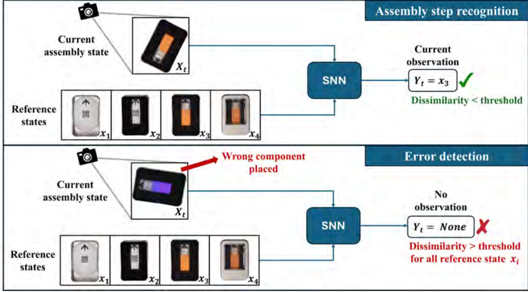
Figure 1.: SNN-based assembly step recognition and error detection mechanisms.
