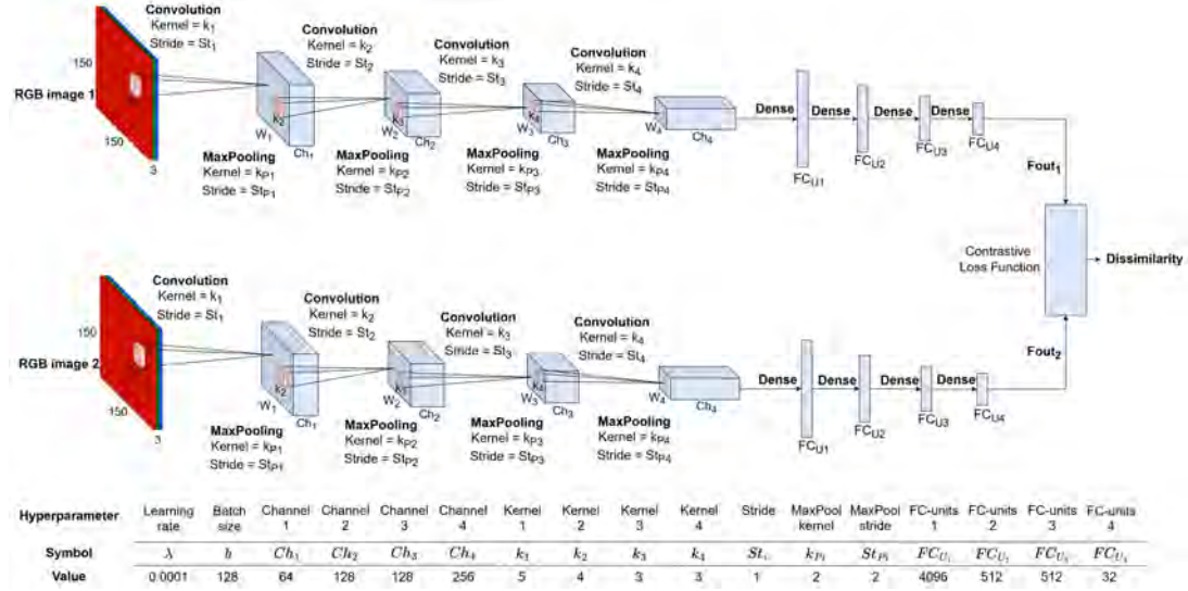
Figure 2.: Siamese Network's architecture: two parallel Convolutional Neural Networks with four convolutional layers with kernel k_i , stride St_i and channel number Ch_i , four max-pooling layers with kernel k_{P_i} and stride St_{P_i} and four fully connected layers with FC-units FC_{U_i}
