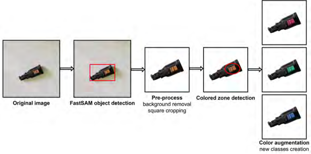
(a) Dataset creation process: FastSAM-based pre-processing of the original image and color data augmentation.
