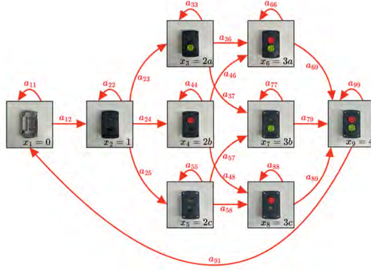
Figure 7.: Feasible transitions between hidden states of the push-button panel assembly
