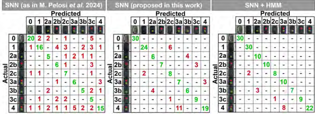
Figure 9.: Confusion matrices for step recognition tests with 10 different operators
