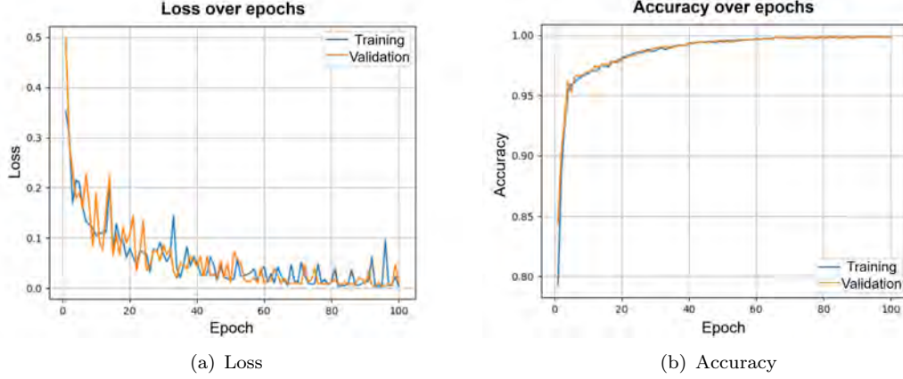
Figure 4.: Training and validation curves for hyperparameters reported in Figure 2
