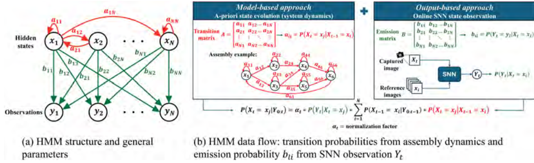
Figure 5.: Hidden Markov Model architecture and data flow
