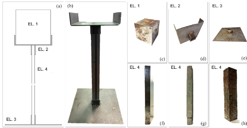
Fig. 4. Experimental setup: (a) Setup design, (b) Iron framework, (c) Steel cube, (d) Upper iron plate, (e) Lower iron plate, (f) Steel column, (g) Concrete column, and (h) Masonry column.
