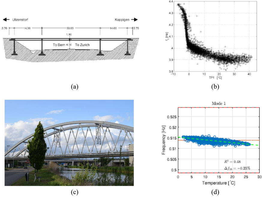
Fig. 1 Relation between frequencies and temperature for bridges from [5] and [4] : (a) Z24 bridge, (b) frequency-temperature scatter-plot, (c) KW51 steel bridge, and (d) frequency-temperature scatter-plot.
