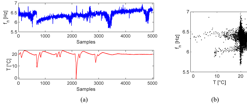
Fig. 7. Results for setup (II) (concrete): (a) Time series of natural frequency and temperature, and (b) natural frequency and temperature scatter plot
