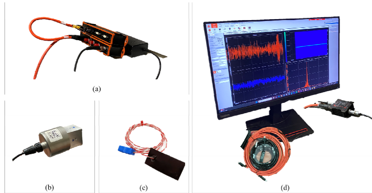
Fig. 5. Sensors and acquisition system: (a) Static (up) and dynamic (bottom) acquisition unit, (b) Accelerometer, (c) Thermometer, and (d) PC and cables
