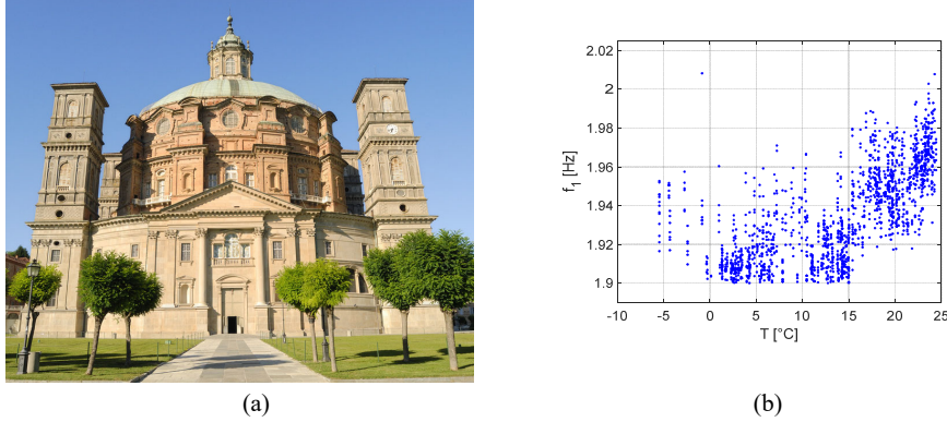
Fig. 3. Relation between frequencies and temperature for Architectural Heritage : (a) the Sanctuary of Vicoforte, and (b) frequency-temperature scatter-plot.
