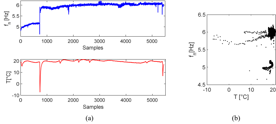
Fig. 8. Results for setup (III) (masonry): (a) Time series of natural frequency and temperature, and (b) natural frequency and temperature scatter plot.
