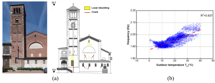
Fig. 2. Relation between frequencies and temperature for Architectural Heritage : (a) Bell tower of Santa Maria del Carrobiolo in Monza [10], (b) frequency-temperature scatter-plot.
