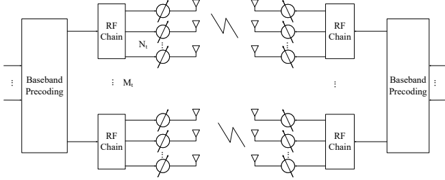
Fig. 2. Partially Connected HBF Architecture.
