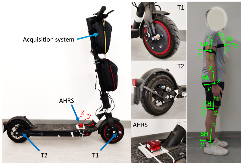
Fig. 6 Sensor setup
