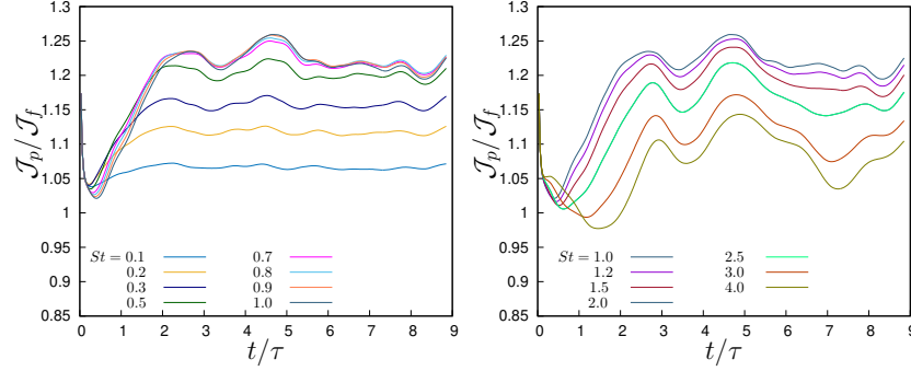
Fig. 3 Integral flux ratio \mathcal{I}_p/\mathcal{I}_f for (a) particles with St \leq 1 ; (b) particles with St \geq 1 .
