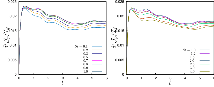
Fig. 2 Integral flux to mean temperature moment ratio, \delta^2 \mathcal{I}_p / \mathcal{I}_f , for (a) particles with St \leq 1 ; (b) particles with St \geq 1 .
