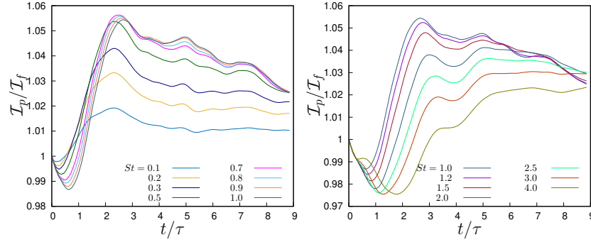
Fig. 1 Mean temperature moment ratio I_p/I_f for (a) particles with St \leq 1 ; (b) particles with St \geq 1 .
