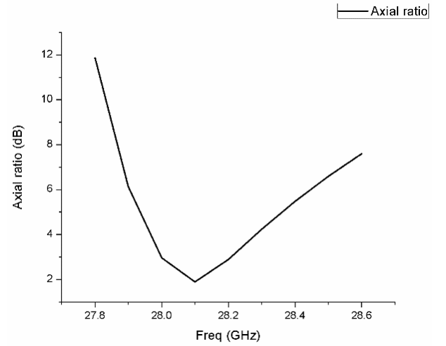
Figure 3. Axial ratio graph for lower band (28 GHz)
