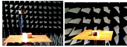
Fig. 14 Measurement setup in an anechoic chamber
