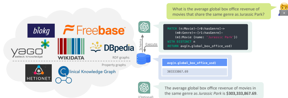
Figure 1: An illustration of Cypher as a unified interface for RDF and property graphs. A graph retrieval for RAG workflow involves: 1) text-to-Cypher translation, 2) query execution, and optionally, 3) final response generation.
