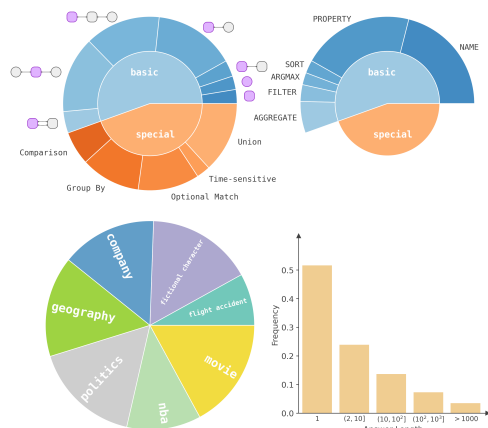
Figure 3: Distribution of graph matching patterns, RETURN templates, domains, and answer lengths (number of rows in the answer) in the CypherBench test set.
