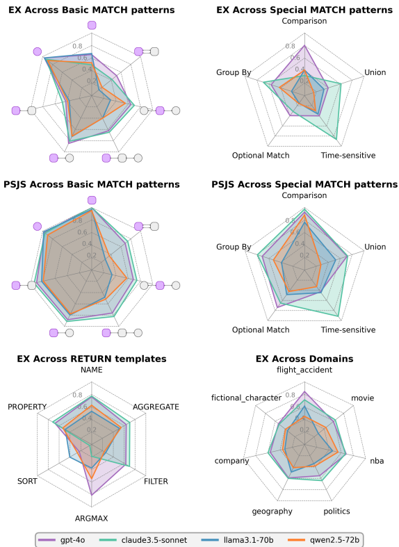
Figure 5: Performance across basic and special MATCH patterns, RETURN templates and domains.
