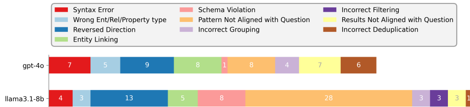
Figure 4: Distribution of errors made by gpt-4o and llama3.1-8b on 50 randomly sampled incorrect predictions. Note that a model might make multiple errors on one instance.
