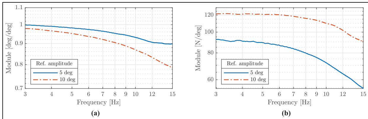
Figure 15. Experiment: Frequency response function of (a) the valve spool position and (b) the actuator output force when applying a sinusoidal spool position reference sweep from 3 to 15 Hz at 5° and 10° of amplitude. The hydraulic actuator position is locked.
