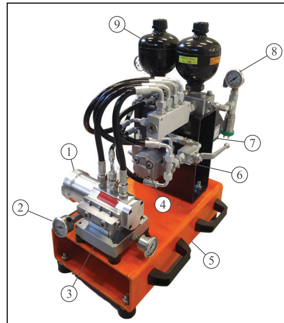
Figure 10. Test bench layout: (1) valve, (2) actuator pressure gage ( \times 2 ), (3) hydraulic manifold, (4) hydraulic pump, (5) frame, (6) pressure-relief valve, (7) electric motor, (8) rail pressure gage ( \times 2 ), and (9) hydraulic accumulator ( \times 2 ).
