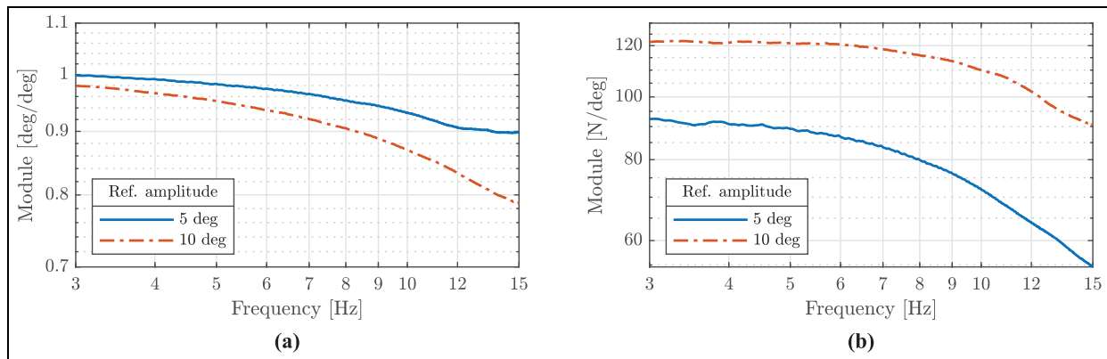
Figure 15. Experiment: Frequency response function of (a) the valve spool position and (b) the actuator output force when applying a sinusoidal spool position reference sweep from 3 to 15 Hz at . and 10° of amplitude. The hydraulic actuator position is locked.
