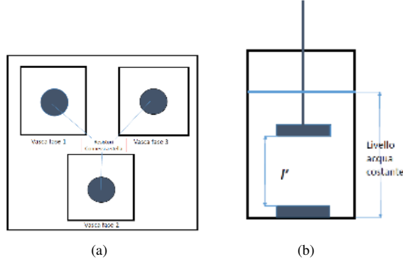
Fig. 4: Simplified sketch of the new dissipating system: (a) top view, (b) front view.
