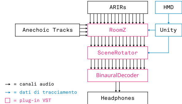
Figure 3: Signal processing chain for dynamic auralization.
