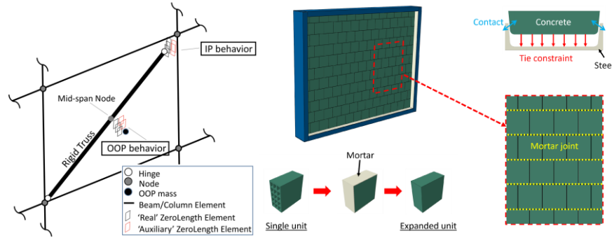
Fig. 4. Numerical modelling strategies: a) macro modelling (modified after Ricci et al., 2018); b) micro modelling.
