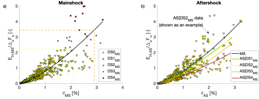
Fig. 1. Hysteretic energy vs maximum inter-storey drift relationship for a case-study RC frame: a) mainshock; b) aftershock (dependent on the damage state in the mainshock). Gentile & Galasso, 2021)
