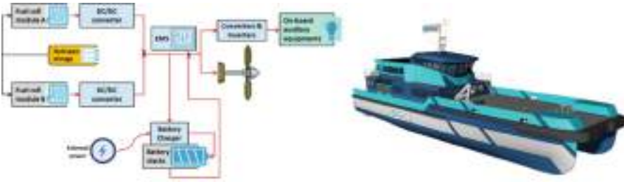
Fig. 1. Crew Transfer Vessel (CTV) case study of Hybrid FC/Battery propulsion system “Source: Authors”.
