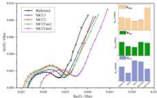
Fig. 3. EIS Nyquist plots responses and values of R_{\text{ohm}} , R_{\text{SEI}} and R_{\text{CT}} for the different cells.
