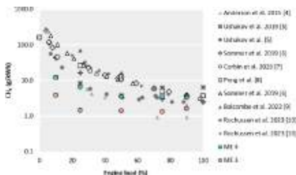
Fig. 1. Methane slip measured on-board a modern diesel-electric Ro-Pax vessel from state-of-the-art engine (ME4) and engine applying a new combustion concept (ME3). Results are compared to other on-board measurements of 4-S LPDF engines [4–10]. Note the logarithmic scale.
