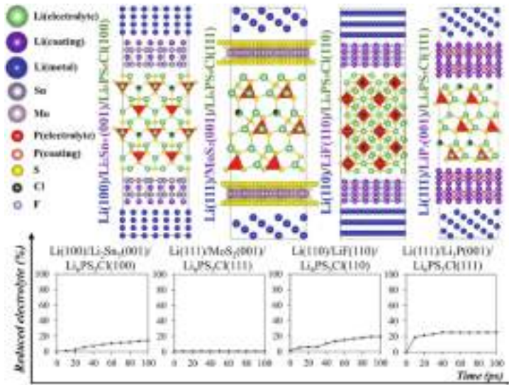
Fig. 5. AIMD simulations of Li/coating/Li 6 PS 5 Cl (image courtesy of CIC energiGUNE, reproduced with permission, The AIMD simulations were performed using the Vienna Ab Initio Simulation Package -VASP)
