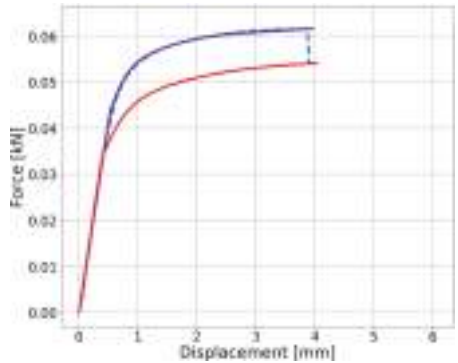
Fig. 2. Simulation data with experimentally extracted model (red), optimized simulation data (purple) and experimental data (dashed blue). Source: Authors
