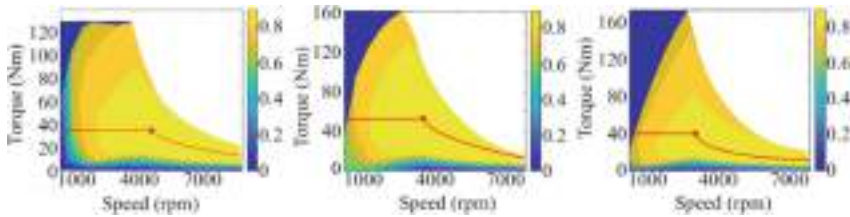
Fig. 2. Nominal torque-speed curve (red line) and efficiency map of Motor 1 (left), Motor (middle), and Motor 3 (right). Source: Authors.
