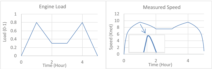
Fig. 5. a) Workboat operational profile i.e., engine load target. b) Workboat’s resulting speed based on its operational profile.
