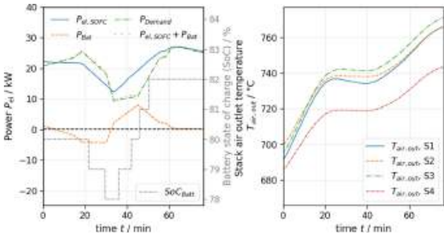
Fig. 3. Experimental results of the laboratory proof of concept at DLR with SolydEra 32 kW LSM and 40 kWh Li-Ion Battery with implemented hybrid genset control strategy given by EMS developed by RWTH.
