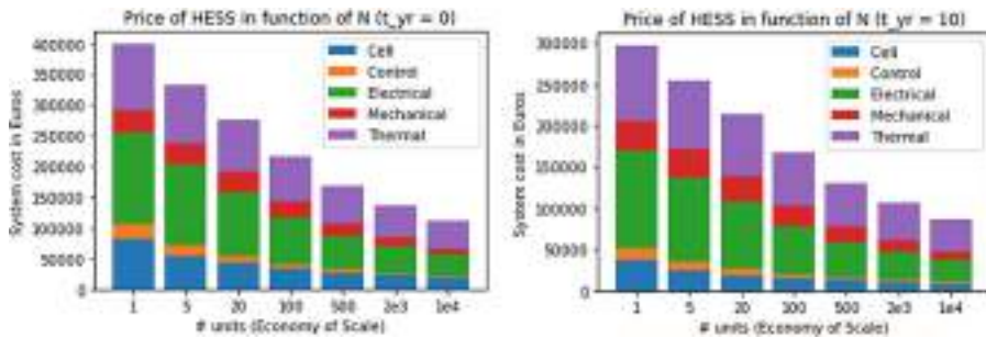
Fig. 4. System cost depending on production volume in present (left) and 10 years (right)
