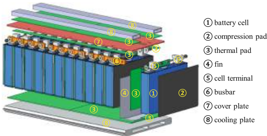
Fig. 1. Explosion view of the module thermal management system. Reproduced with permission from [AVL Deutschland GmbH], copyright [AVL Deutschland GmbH], [2024].
