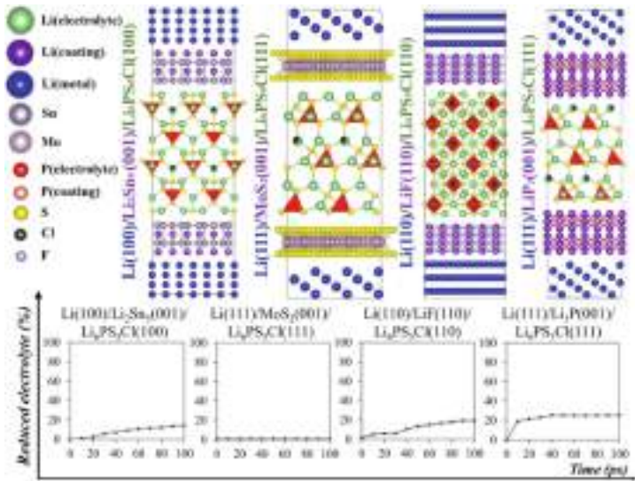
Fig. 5. AIMD simulations of Li/coating/ \text{Li}_6\text{PS}_5\text{Cl} (image courtesy of CIC energiGUNE, reproduced with permission, The AIMD simulations were performed using the Vienna Ab Initio Simulation Package -VASP)
