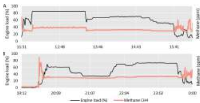
Fig. 3. Methane concentrations measured on-board modern Ro-Pax ferry from engine piloting new combustion concept (ME3) during two voyages Umeå-Vaasa (A) and Vaasa-Umeå (B).
