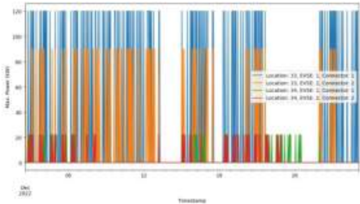
Fig. 4. Max. Power per EVSE and hour.
