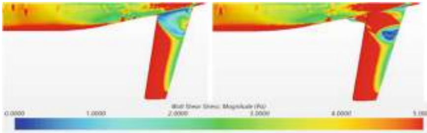
Fig. 2. Contour of wall shear stress (Pa) at M = 0.2 , sea level, AoA = -10 deg. Deep blue regions represents separated flow. FSHTP without (left) and with LEX, (right). Picture generated with ANSYS®.
