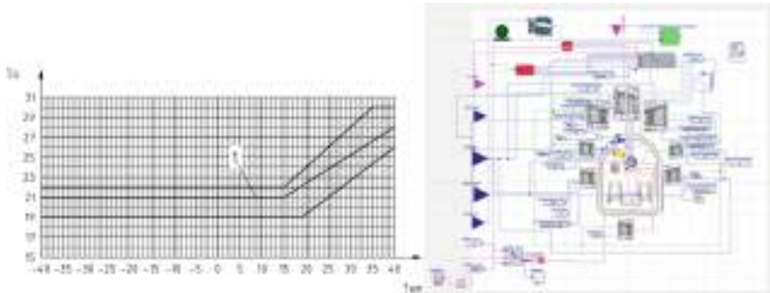
Fig. 2. Left: Set point for the temperature in °C in the passenger compartment ( T_{ic} ) as a function of the outside temperature ( T_{em} ) in °C – Upper, recommended (1) and lower curve of DIN EN 14750, Right: Dymola surface of the thermal car body model (TCBM)
