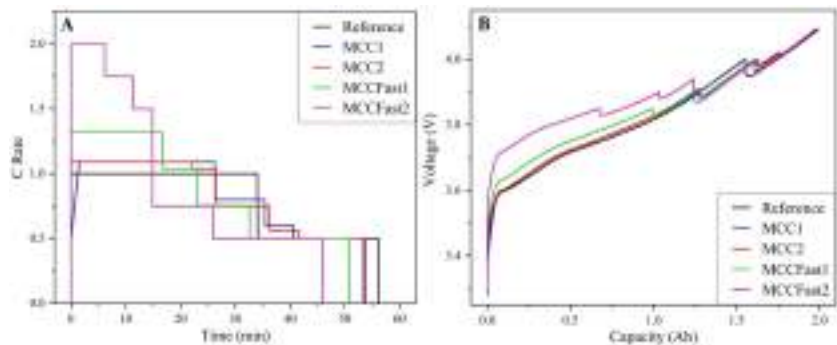
Fig. 1. (A) C-Rate vs Time charging profiles and (B) Voltage response vs Capacity charging profiles.
