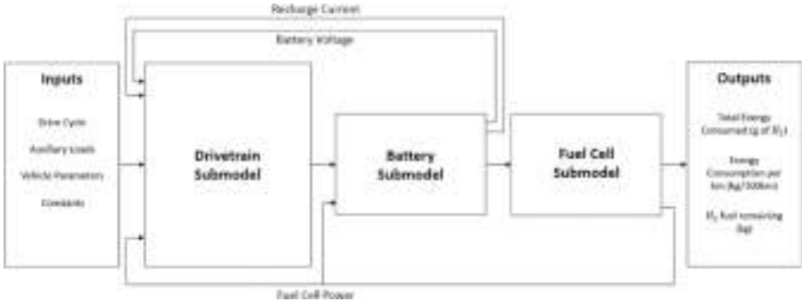
Fig. 1. Schematic of Fuel Cell Electric Vehicle Simulation including model inputs and outputs.
