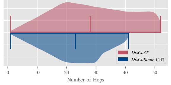
Fig. 5. Hop Count distribution: DisCo3T vs. DisCoRoute (4T).
