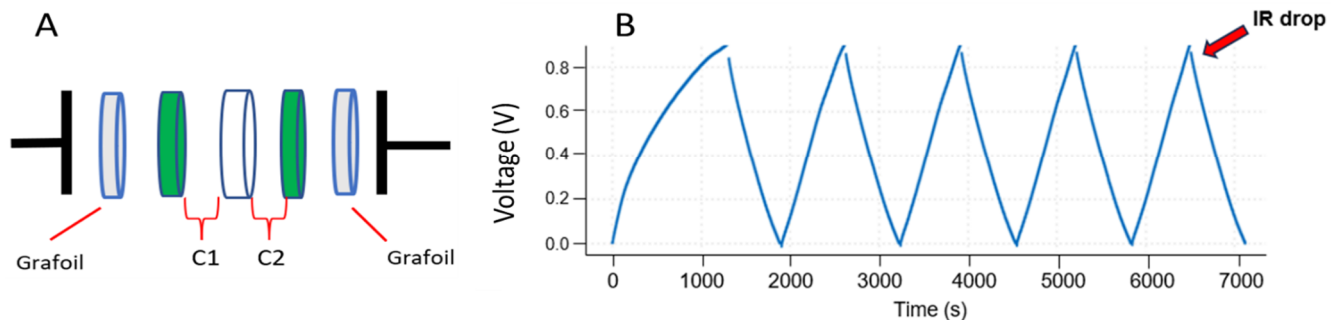
Figure 4. (A) Symmetric cell assembly with Grafoil collectors; (B) GCD curves.
