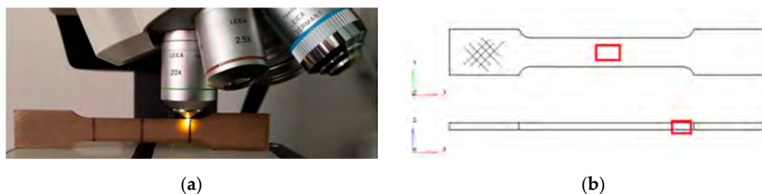
Figure 3. (a) Experimental setup to perform confocal microscopy on the lateral surface of the specimen; (b) highlighted areas analyzed by the microscope in the xy- and xz-planes.
