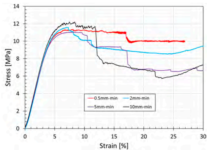
Figure 8. Stress–strain curves obtained from compressive tests performed on cubic gyroid specimens ( 30 \times 30 \times 30 \text{ mm}^3 ) at different test speeds.
