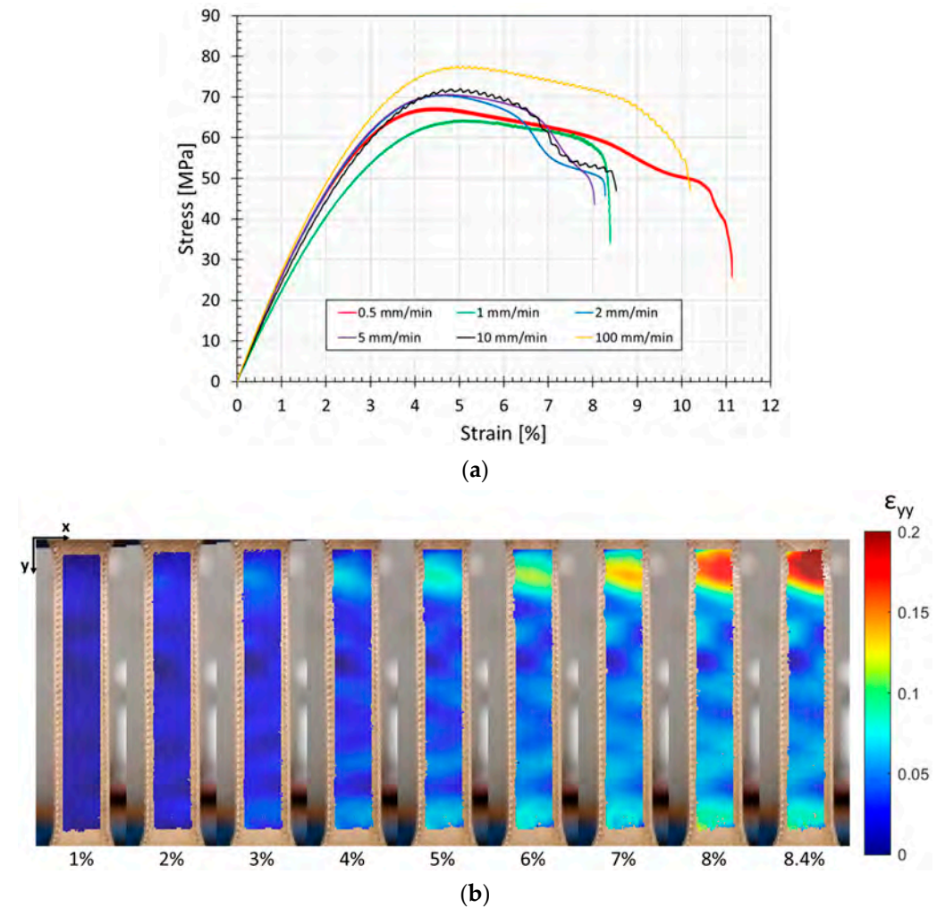
Figure 6. (a) Tensile test results: stress–strain curves; (b) explanatory strain distribution obtained through DIC analysis, performed for sample tested at 1 mm/min. The color bar reports the strain values along the y -axis direction; the percentage values beneath the strain maps indicate the corresponding strain value of the stress–strain curve.
