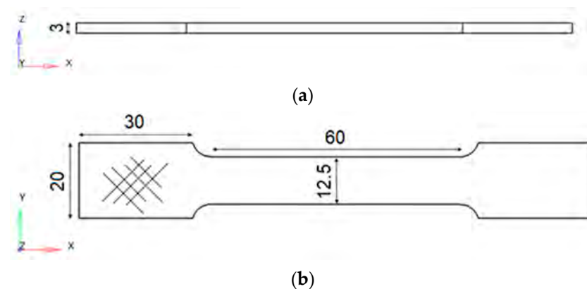
Figure 1. Tensile test specimen. (a) View of the xz-plane; (b) view of the xy-plane; the raster angle is visible on the left side.
