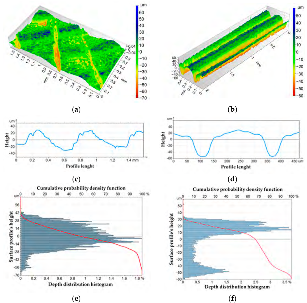
Figure 4. Surface topography of tensile specimen: upper surface (a) and lateral surface (b). Rugosity profiles of upper surface (c) and lateral surface (d). Abbott–Firestone curves of upper surface (e) and lateral surface (f). The red curves in (e,f) are the cumulative probability density functions.
