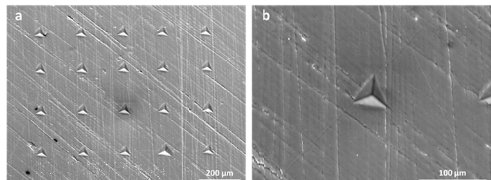
Figure 13. SEM images of nanoindentation imprints: (a) 4 \times 5 indentation matrix; (b) representative indentation imprint.
