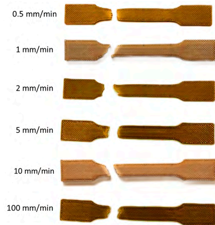
Figure 7. Specimens tested during tensile tests.
