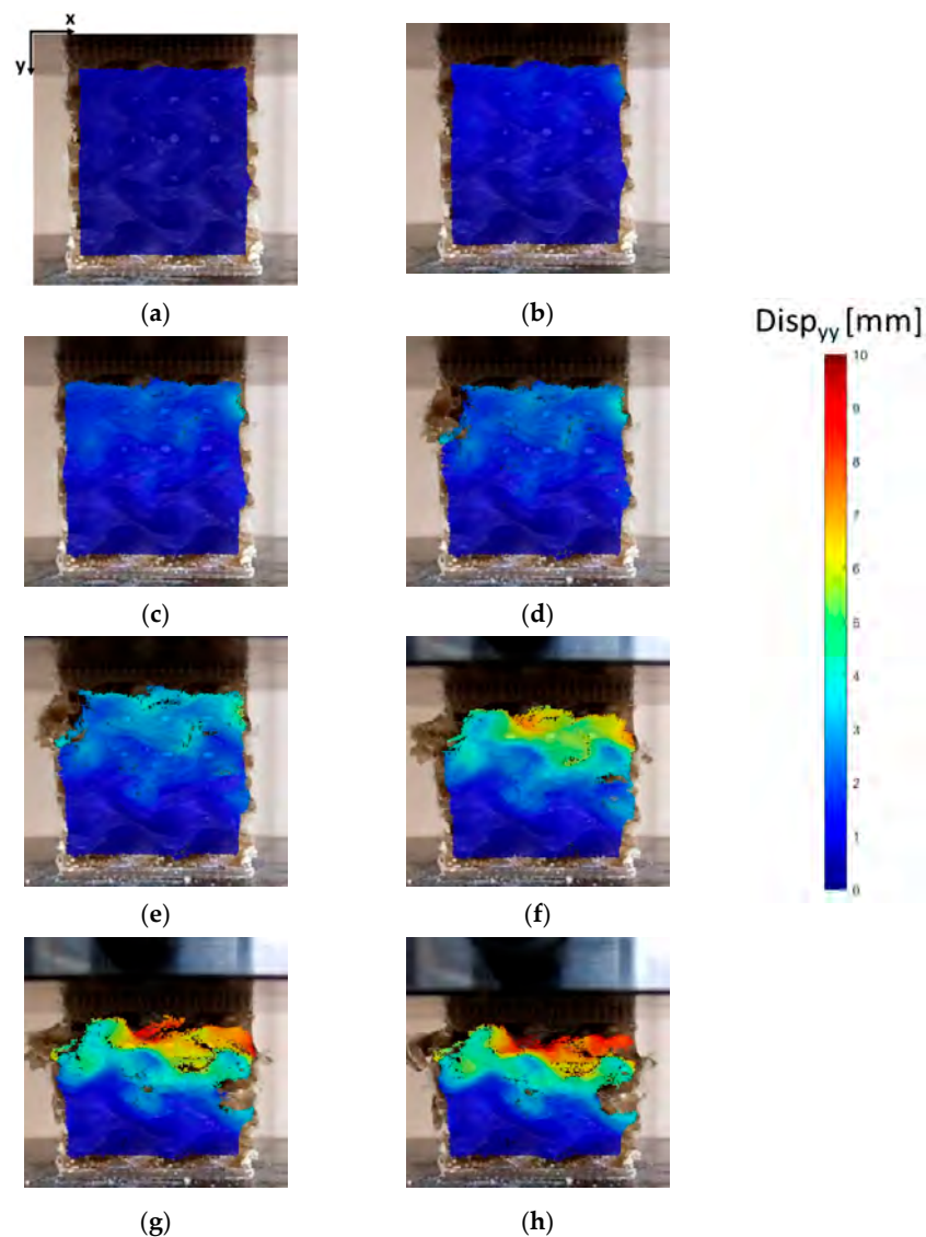
Figure 9. Vertical displacements calculated using the DIC technique for the specimen subjected to a compression test at 2 mm/min. The panels from (a–c) represent the distribution of displacement
