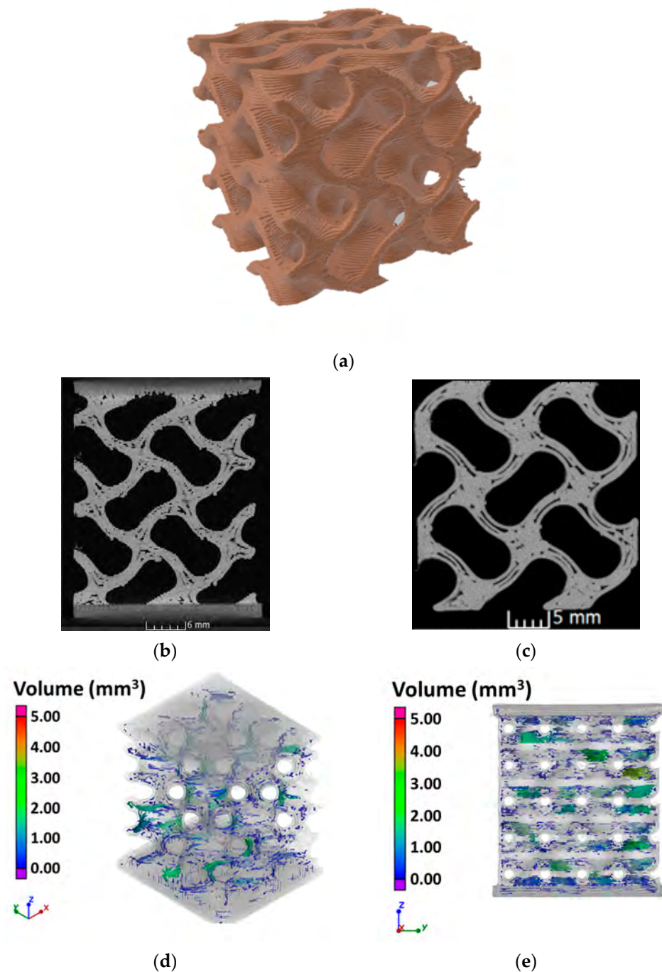
Figure 5. (a) Volumetric reconstruction of the specimen; (b,c) slices showing internal defects; (d,e) counts of defects' volume.
