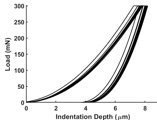
Figure 11. Load–displacement curves obtained from nanoindentation tests. Loading/unloading rates were set at 15 mN/s, imposing 20 s of holding time at the prescribed load value.
