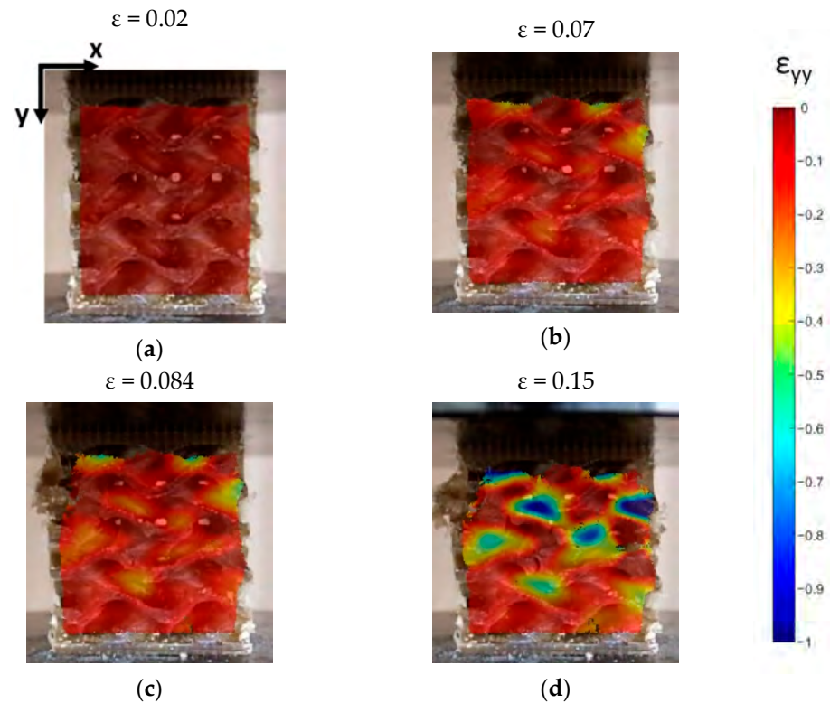
Figure 10. Vertical strain distribution calculated by DIC for the specimen subjected to compression test at 2 mm/min. The images refer to the following phases: (a) elastic phase; (b) strain at maximum load; (c) strain at the load drop after the maximum load; (d) plateau region.
