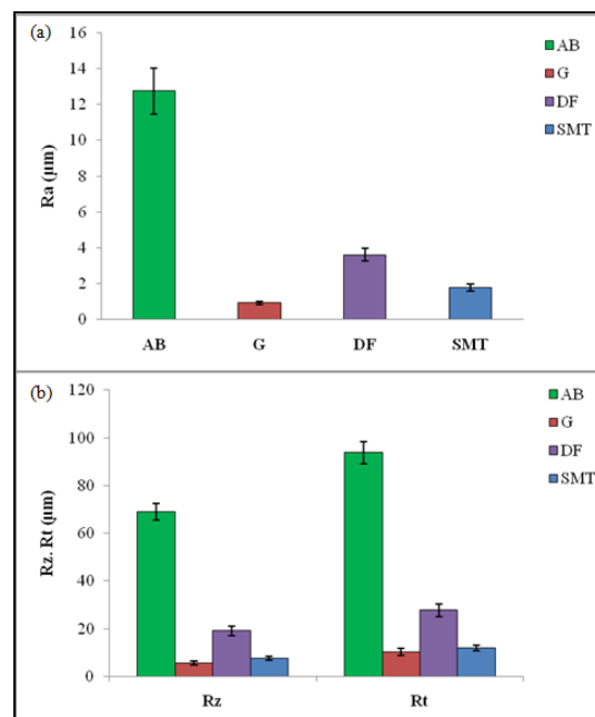
Fig. 3. Surface roughness parameters of the AB Ti6Al4V manufactured by EBM and after (G), (DF) and (SMT).
