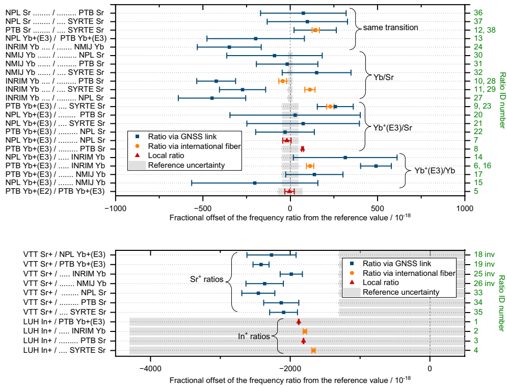
Fig. 2. Frequency ratios measured in March 2022 via GNSS links (blue squares), international fiber links (orange circles), and local comparisons (red triangles). The error bars on the data points represent the total relative standard uncertainties for each measurement, including statistical and systematic uncertainties. The gray bars show the relative standard uncertainties on the reference frequency ratios, which are obtained from the least-squares adjustment of standard frequencies, approved by the International Committee for Weights and Measures (CIPM) in 2021 and reported in Table S1 of Supplement 1. The right-hand axis of the plots shows the ratio ID numbers, corresponding to the rows in Table 2 that give the measured values of the frequency ratios; the ID numbers are marked with “inv” if the ratio is inverted between the graph and the table.
