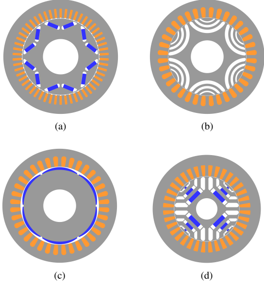
Fig. 1. Cross-sections of the four benchmark machines: a) IPM, b) SyR, c), SPM and d) PM-SyR.
