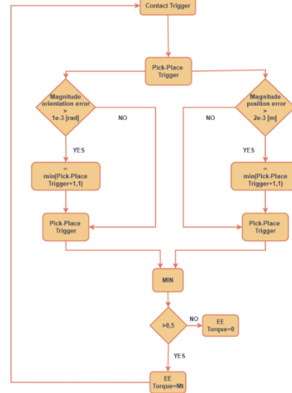
Figure 3, Grasping algorithm
