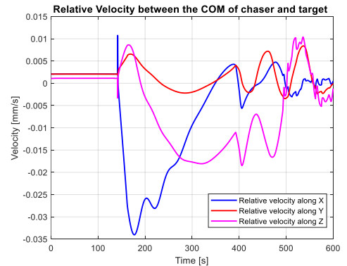
Figure 7, Relative velocities during berthing process.
