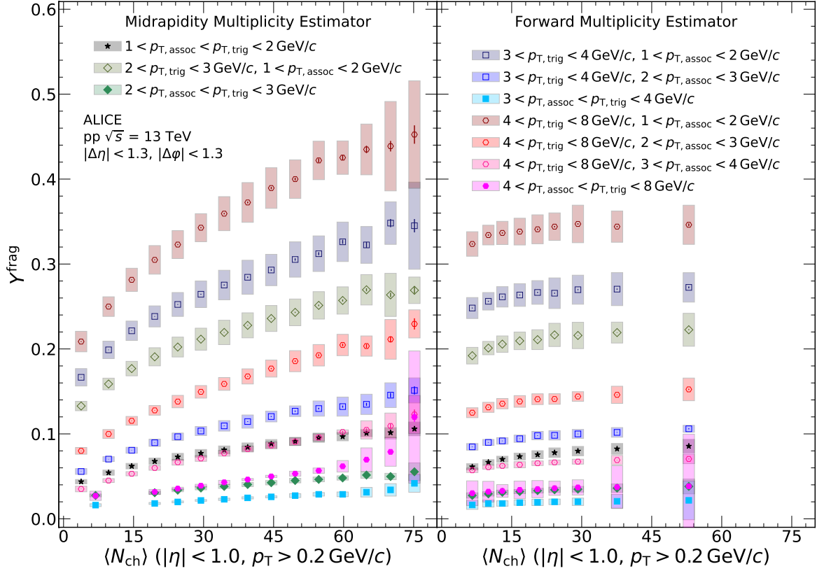
Figure 4. Per trigger normalised yield of associated particles in the near-side as a function of \langle N_{\text{ch}} \rangle for all p_{T, \text{trig}} and p_{T, \text{assoc}} intervals. Results with event activity measured at midrapidity (forward rapidity) are shown on the left (right). The statistical and systematic uncertainties are displayed with error bars and boxes, respectively.
