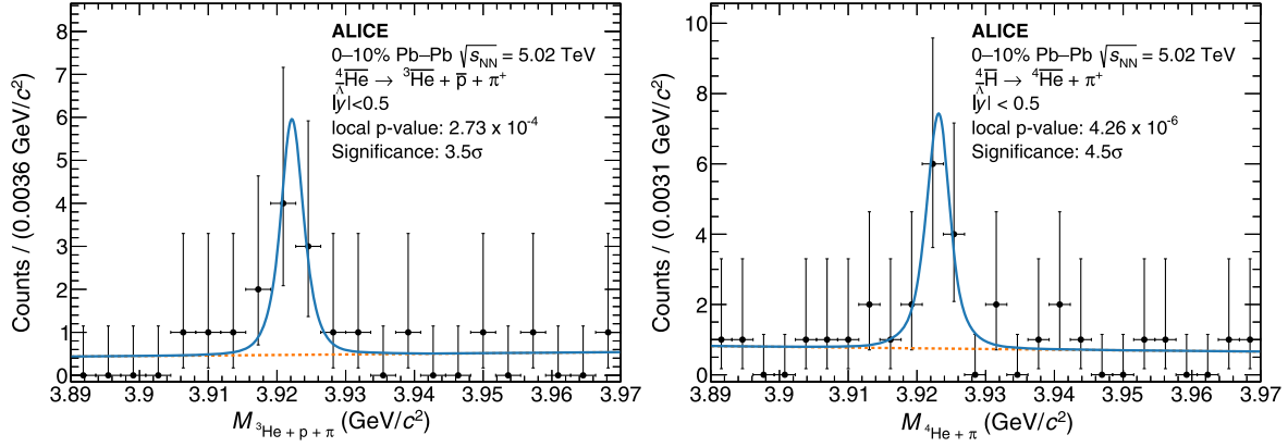
FIG. 1. Invariant-mass spectra of \bar{\Lambda}^3\text{He} candidates on the left and \bar{\Lambda}^4\text{He} candidates on the right. These spectra are fitted with a KDE template for the signal peak (blue curve) and an exponential function to model the background (orange curve). The combined invariant-mass spectra for the sum of particle and antiparticle states of each (anti)hypernucleus are shown in the End Matter.
