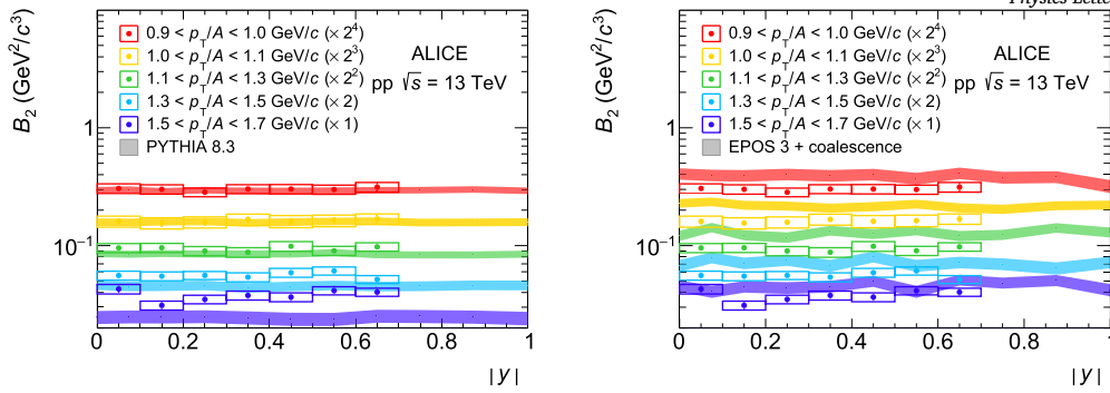
Fig. 4. Coalescence parameter B_2 as a function of rapidity, for fixed transverse momentum per nucleon values. Statistical and systematic uncertainties on the data points are represented by vertical bars and boxes, respectively. The statistical uncertainties are smaller than the size of the markers in the reported scale and, hence, not visible. Bands show the model predictions from PYTHIA 8.3 (left panel) and from a coalescence model [57] used as afterburner of EPOS 3 (right panel), the width reflecting the statistical uncertainties.
