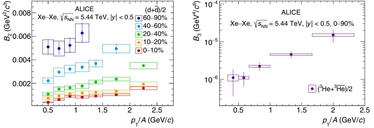
FIG. 6. Coalescence parameters B_2 (left panel) and B_3 (right panel) as a function of p_T/A , measured for deuterons and {}^3\text{He} , respectively. Statistical uncertainties are represented as vertical lines whereas boxes represent the systematic ones.
