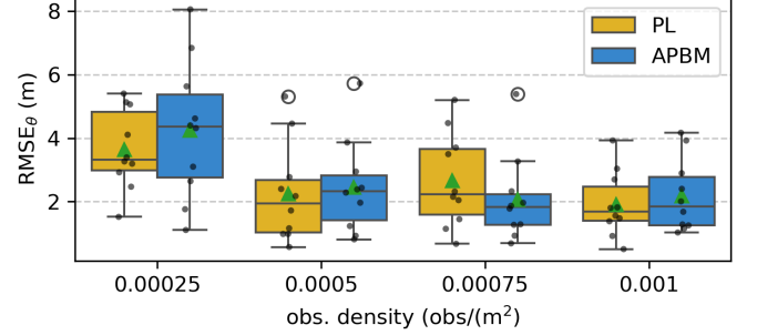
(a) Open-sky path-loss scenario.
