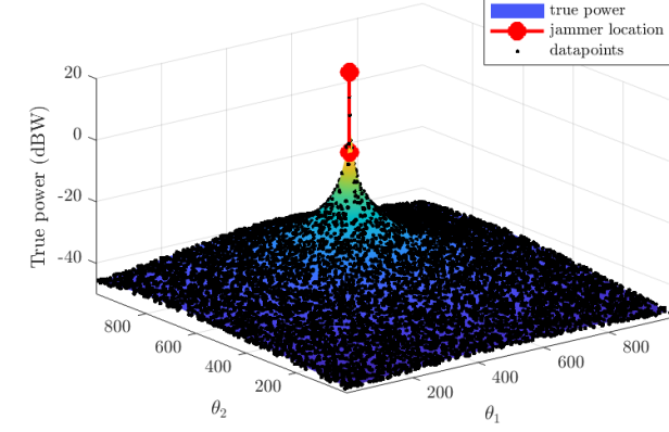
(a) Open-sky path-loss scenario.
