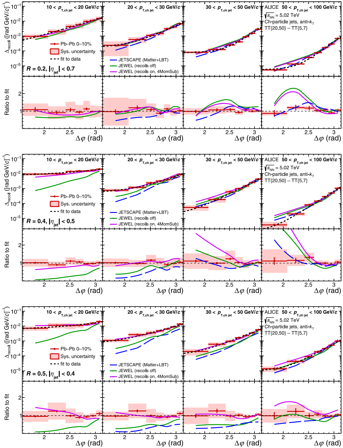
FIG. 14. Corrected \Delta_{\text{recoil}}(\Delta\phi) distributions for Pb-Pb collisions at \sqrt{s_{\text{NN}}} = 5.02 TeV, for R = 0.2 (top), 0.4 (middle), and 0.5 (bottom) in p_{T, \text{ch jet}} bins (left to right): [10, 20] , [20, 30] , [30, 50] , and [50, 100] GeV/c. JETSCAPE and JEWEL calculations are also shown. Upper subpanels show the individual distributions, while lower subpanels show their ratio to a functional fit of the data.
