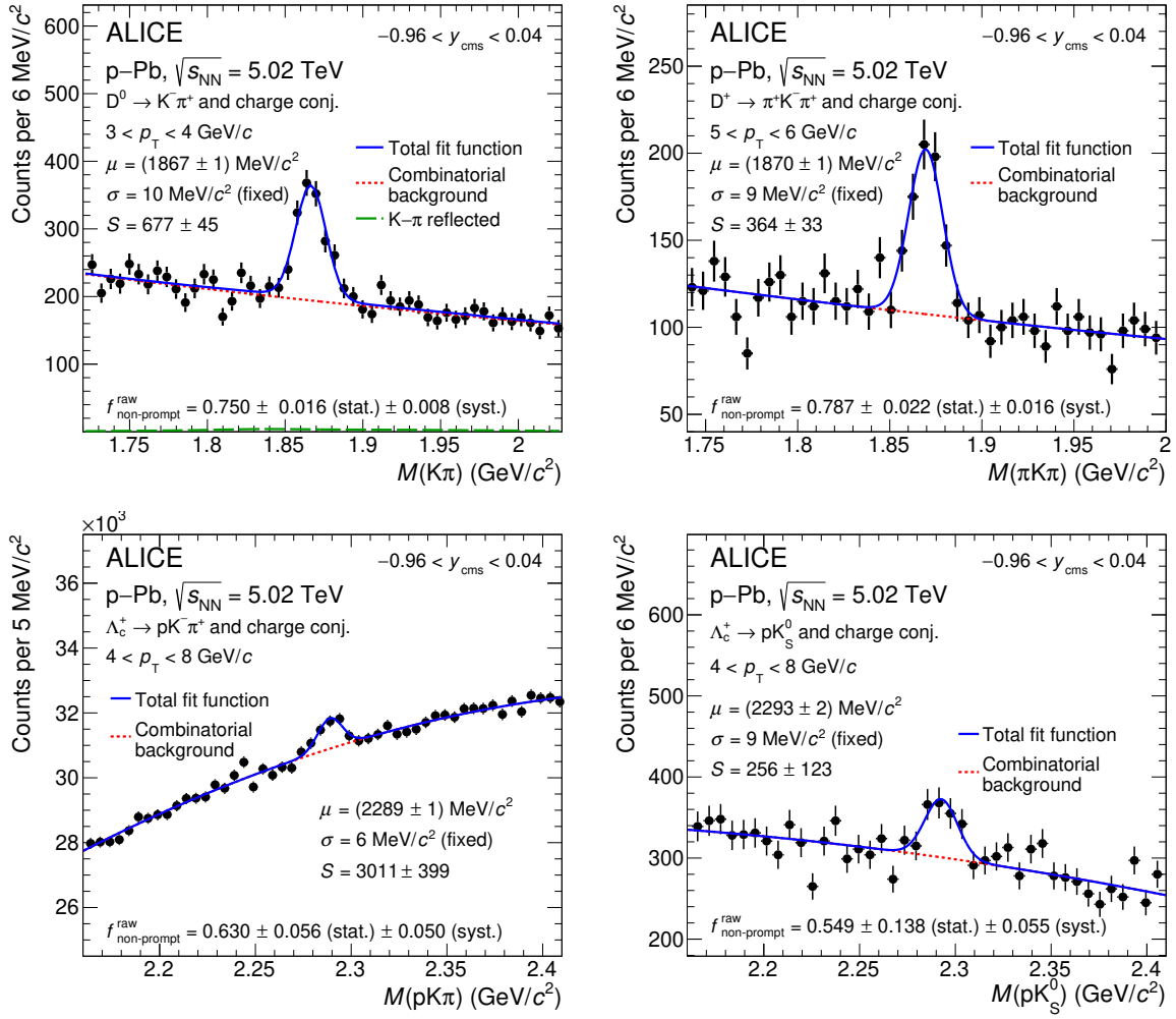
Figure 1. Invariant-mass distributions of D 0 -, D + -, and Λ c + -hadron candidates, and their charge conjugates in selected p_T intervals. The blue solid lines show the total fit functions as described in the text and the red dashed lines show the fit function describing the combinatorial background. For D 0 -meson candidates, the solid green line represents the contribution of the reflections. The mean ( \mu ) and fixed standard deviation ( \sigma ) of the signal fit function, along with the raw-yield ( S ) values, are reported together with their statistical uncertainties resulting from the fit. The fraction of non-prompt candidates in the measured raw yield ( f_{non-prompt}^{raw} ) is reported with its statistical and systematic uncertainties.
