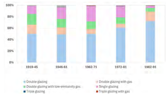
Fig. 4 – Glazing type share per construction period
