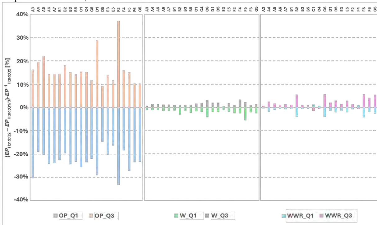
Fig. 5 – Results of the SA. Space heating variation of the city block for different scenarios of the building envelope parameters
