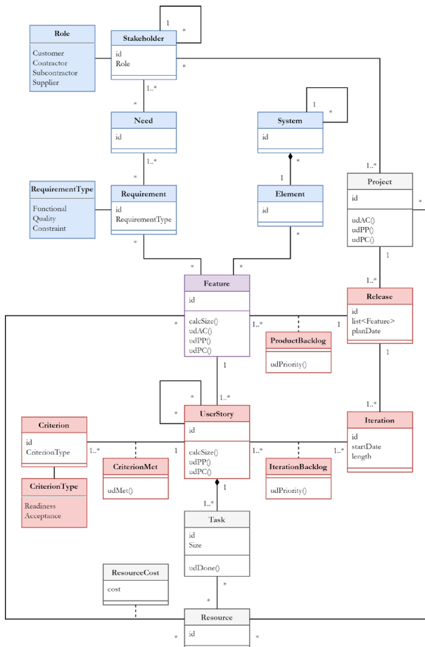
Figure 1: Agile SE and PM integration class diagram
