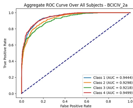
Figure 7. Aggregate ROC curve over all subjects for BCICIV_2a MI dataset: the plot presents the ROC curves for all four classes, showing the model's classification performance across subjects. The AUC values indicate high discriminative ability, with all classes achieving values above 0.92.
