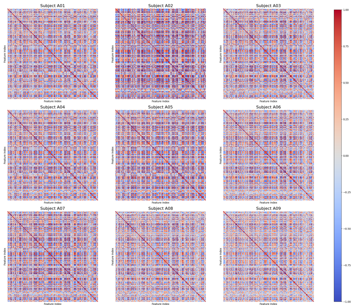
Figure 6. Correlation heatmaps of latent features for each subject of the BCICIV_2a MI Dataset: this figure presents the correlation matrices of latent features extracted from EEG signals for all subjects. The diagonal represents perfect correlation (value = 1), while off-diagonal values indicate varying degrees of correlation between different features. The patterns suggest underlying structure and dependencies in the learned feature representations.
