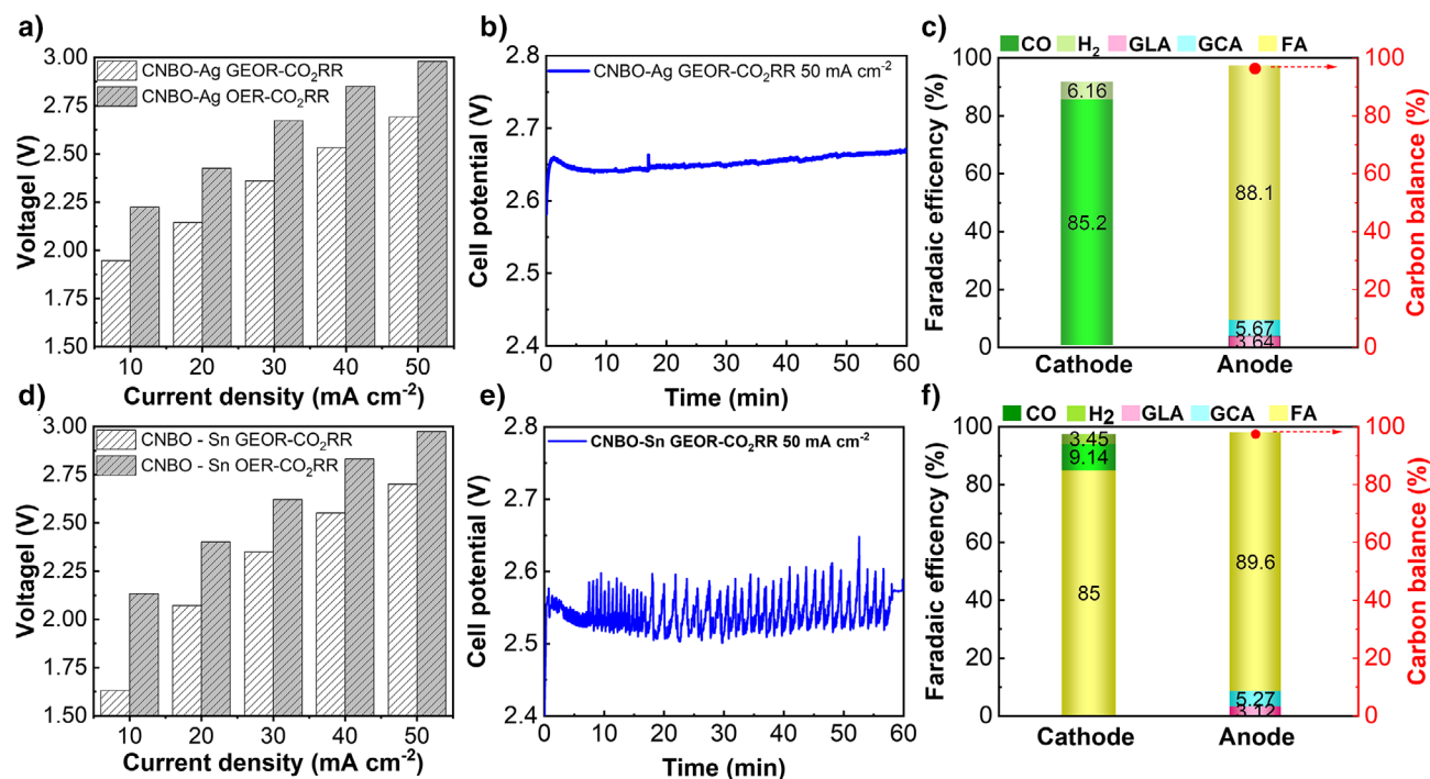
Figure 5. Cell voltage required to achieve specific current densities in different full cells: a) CNBO-Ag/PTFE, d) CNBO-Sn/ Sigracet 39BB. CP scans collected at 50 mA cm -2 implementing b) CNBO + Ag/PTFE, e) CNBO + Sn/Sigracet 39BB configurations, c,f) and related product distribution.
